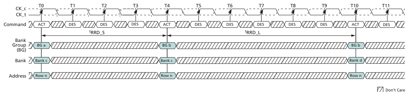
Figure 121: t_{RRD} Timing
