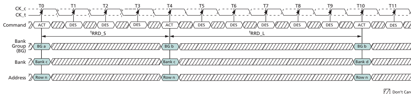
Figure 81: t_{RRD} Timing
