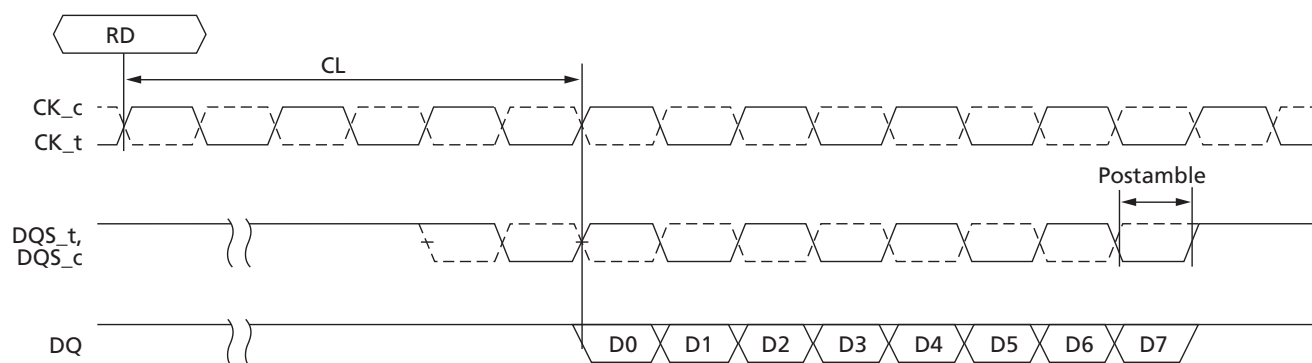
Figure 117: READ Postamble
