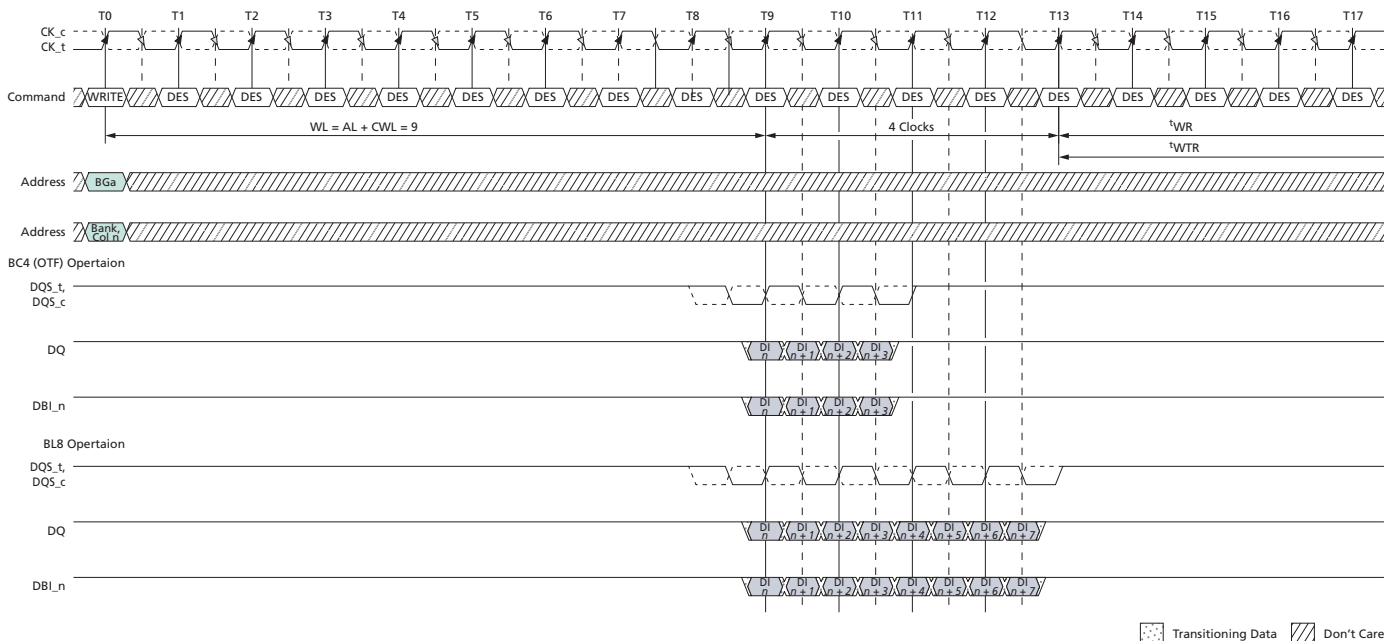
Figure 193: WRITE (BL8/BC4-OTF) with 1^t\text{CK} Preamble and DBI
