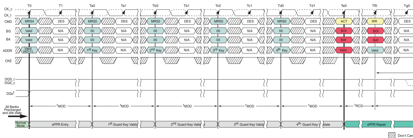
Figure 78: sPPR – Entry
