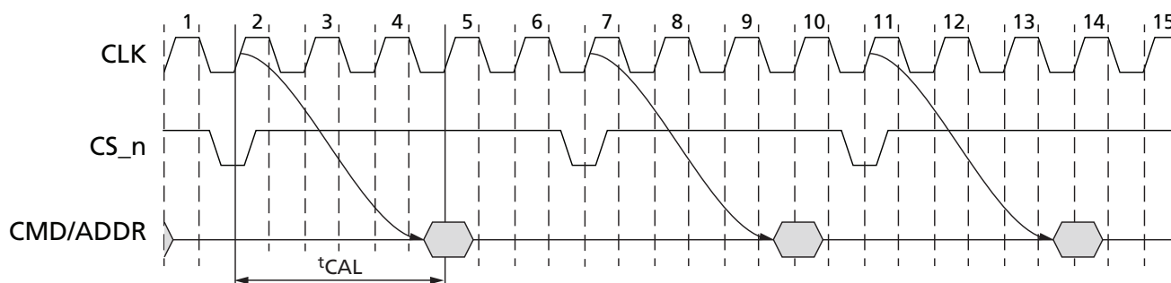
Figure 25: CAL Timing Definition
