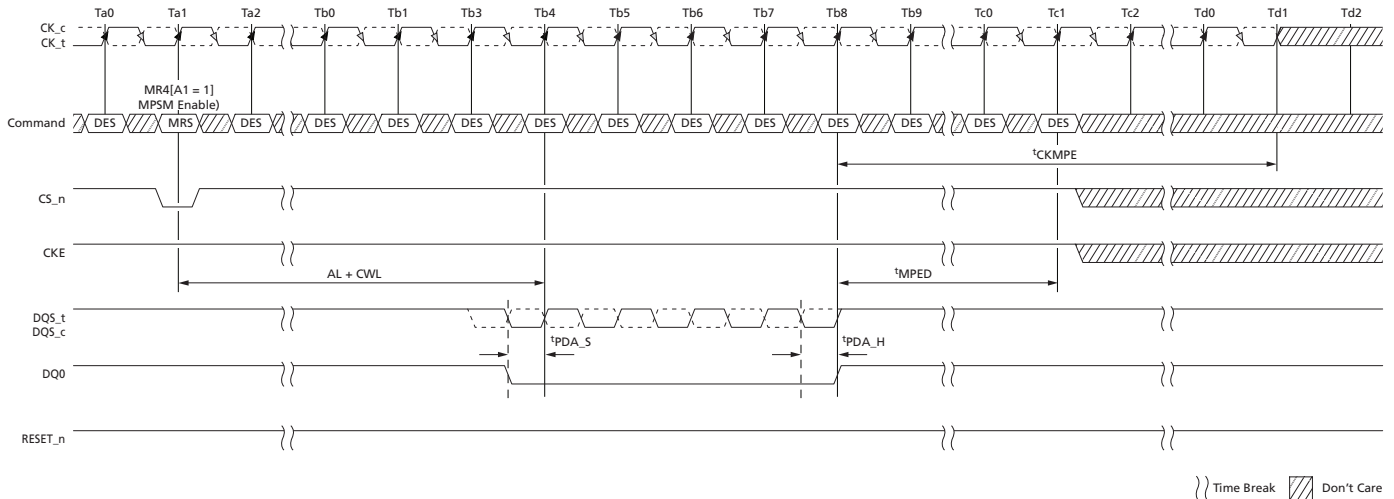
Figure 47: Maximum Power-Saving Mode Entry with PDA
