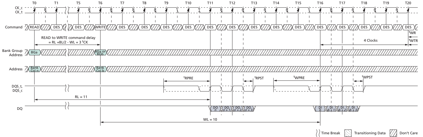
Figure 145: READ (BC4) OTF to WRITE (BC4) OTF with 2 t CK Preamble in Same or Different Bank Group
