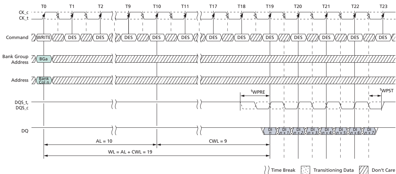
Figure 173: WRITE Burst Operation, WL = 19 (AL = 10, CWL = 9, BL8)
