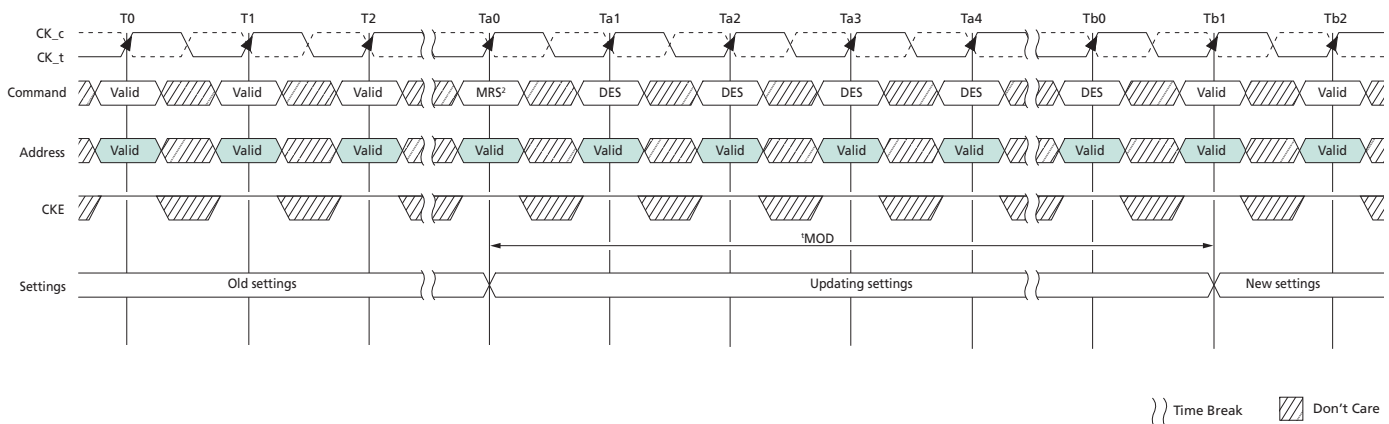
Figure 17: t_{MOD} Timing
