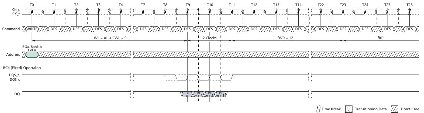
Figure 192: WRITE (BC4-Fixed) to Auto PRECHARGE with 1^t\text{CK} Preamble
