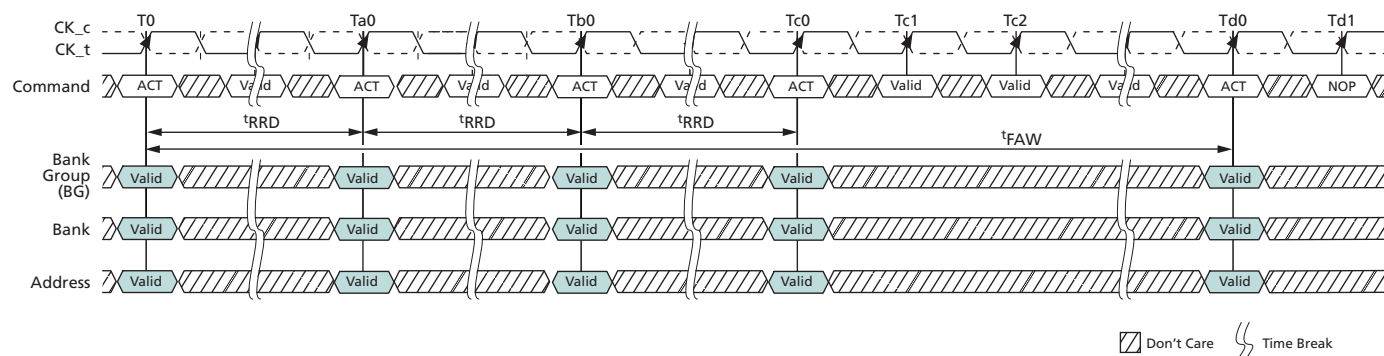
Figure 82: t_{FAW} Timing
