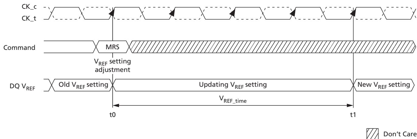
Figure 66: V_{\text{REFDQ}} Timing Diagram for V_{\text{REF,time}} Parameter
