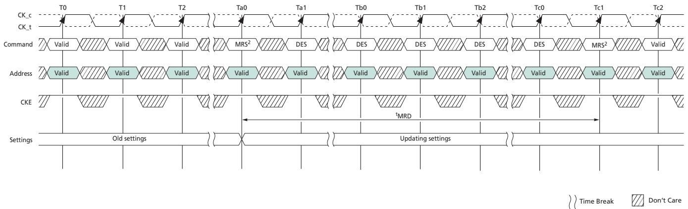
Figure 16: t_{MRD} Timing
