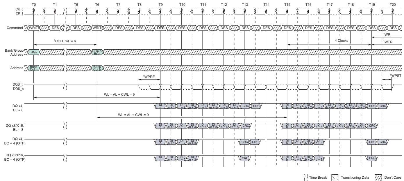
Figure 198: Nonconsecutive WRITE (BL8/BC4-OTF) with 1^t\text{CK} Preamble and Write CRC in Same or Different Bank Group
