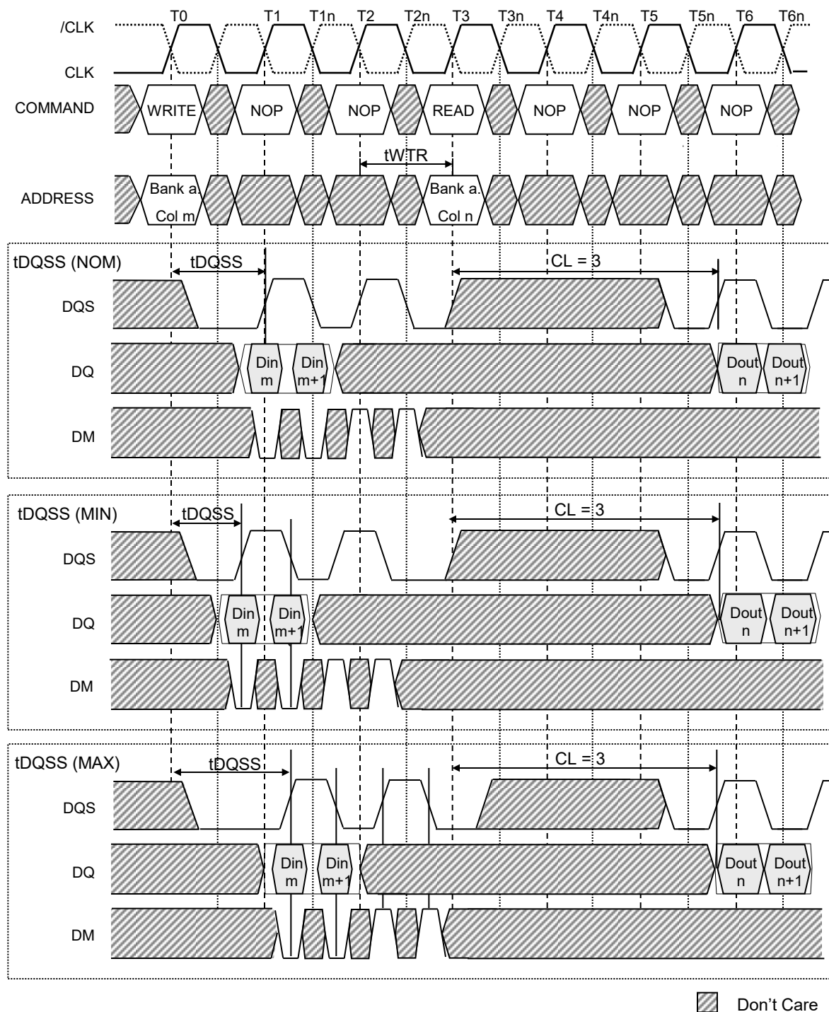
Figure 20: WRITE-to-READ – Interrupting
