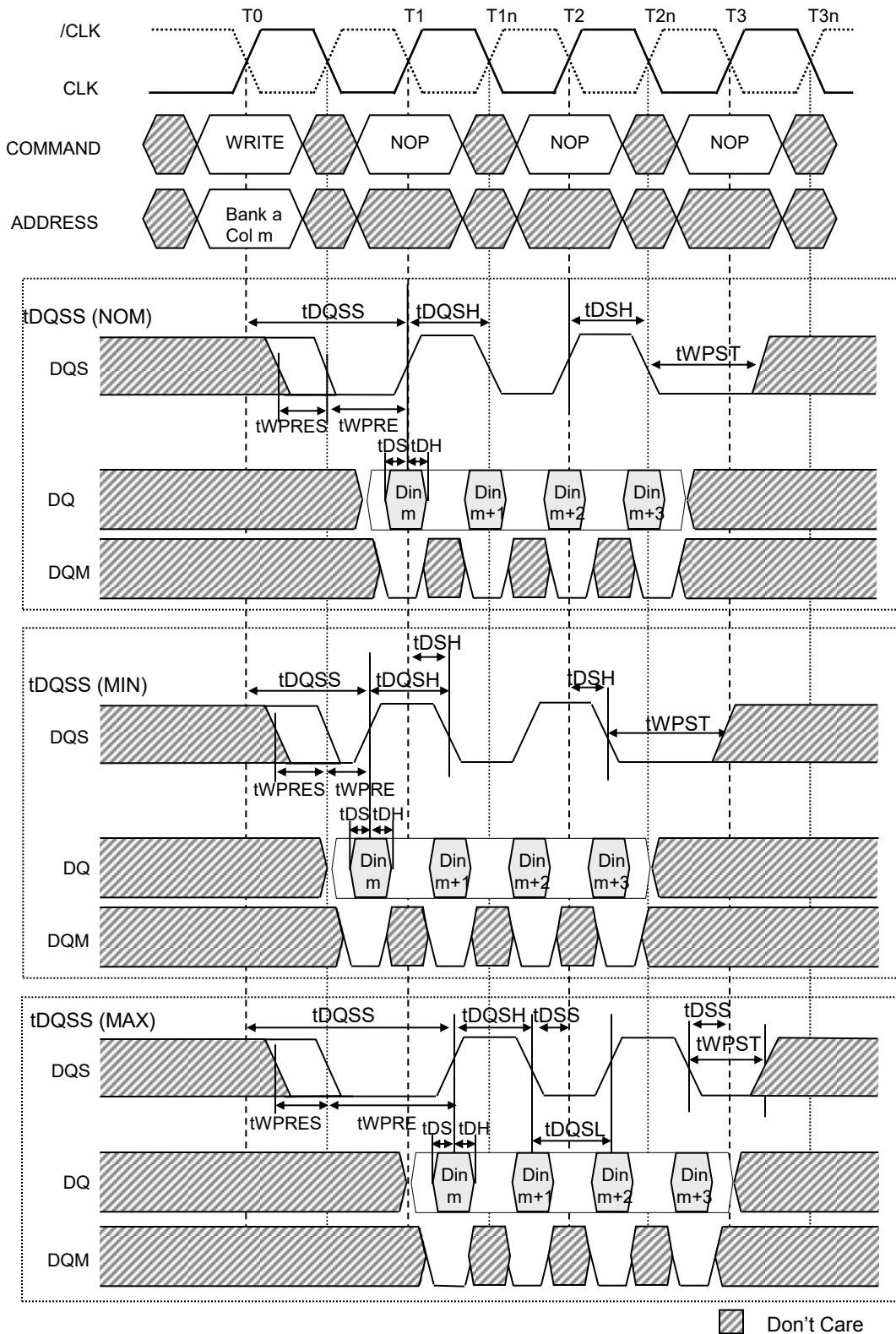
Figure 15: WRITE Operation
