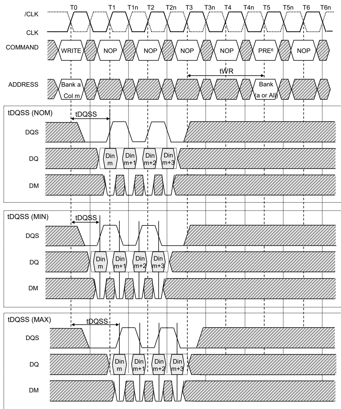
Figure 22: WRITE-to-PRECHARGE – Uninterrupting
