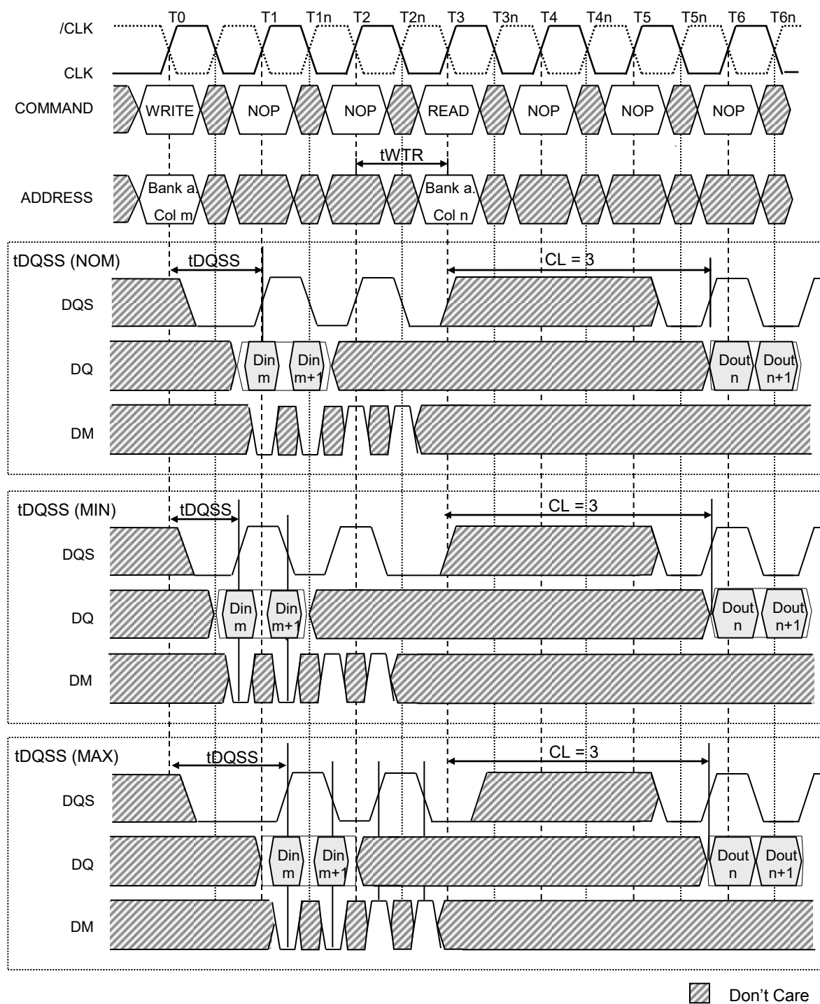
Figure 20: WRITE-to-READ – Interrupting
