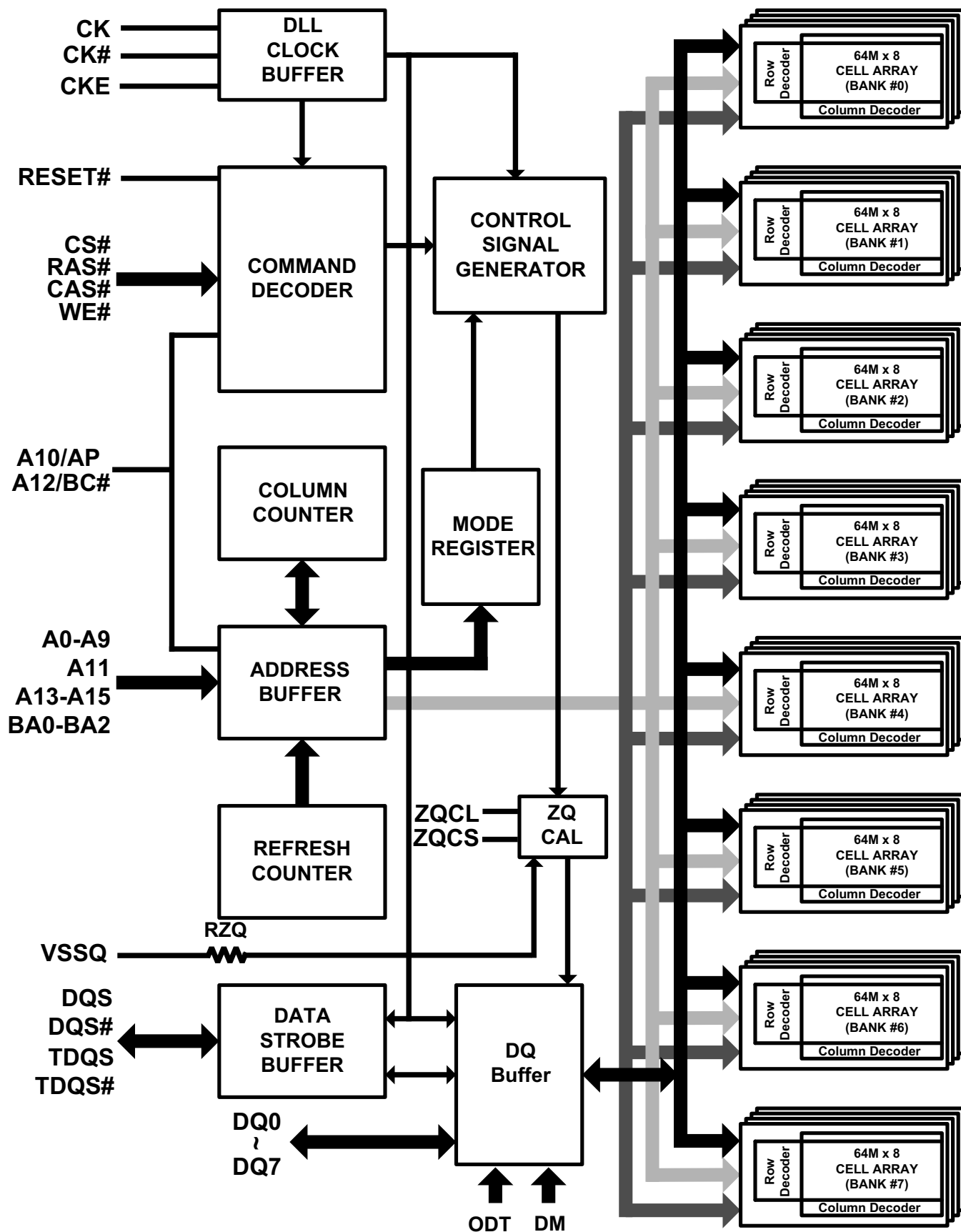
Figure 2. Block Diagram
