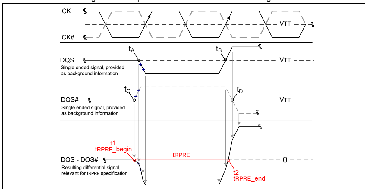
Figure 27 – Method for calculating tRPRE transitions and endpoints
