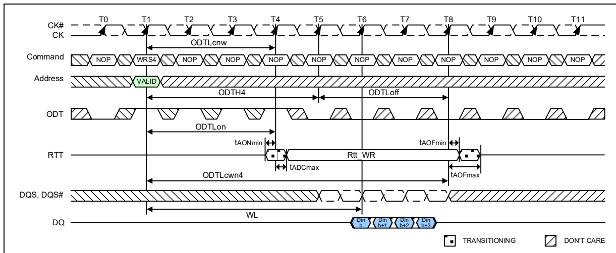
Figure 80 – Dynamic ODT: Behavior with ODT pin being asserted together with write command for duration of 6 clock cycles, example for BC4 (via MRS or OTF), AL = 0, CWL = 5
