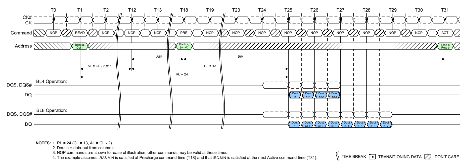
Figure 39 – READ to PRECHARGE (RL = 24, AL = CL-2, CL = 13, tRTP = 6, tRP = 13)
