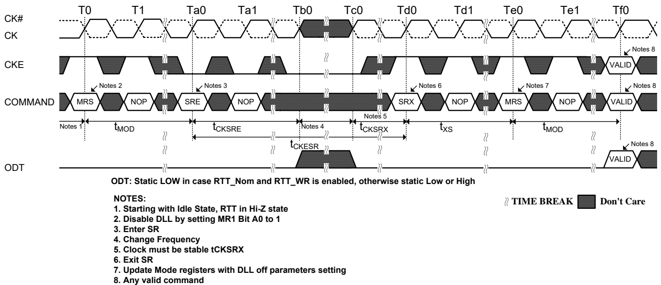
Figure 12. DLL Switch Sequence from DLL-on to DLL-off
