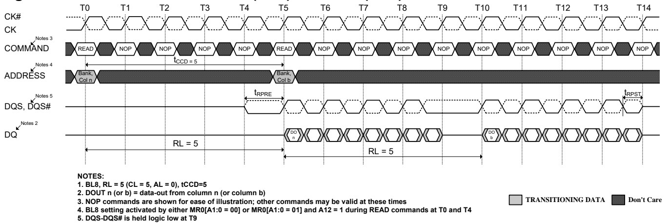
Figure 57. Nonconsecutive READ (BL8) to READ (BL8)
