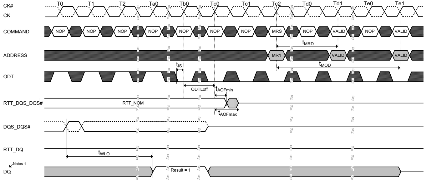
Figure 17. Timing details of Write Leveling exit
