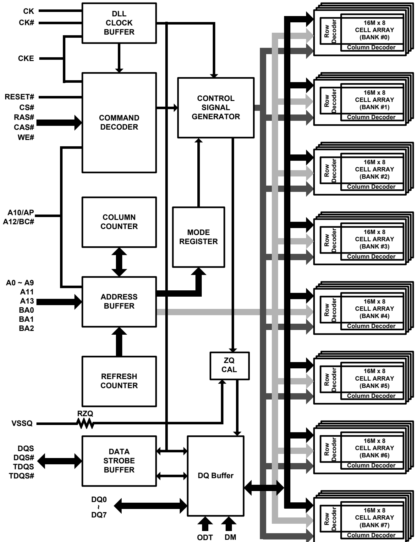
Figure 2. Block Diagram
