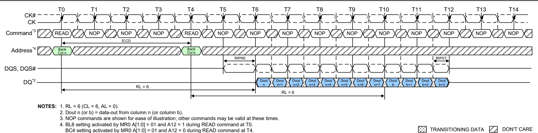
Figure 34 – READ (BL8) to READ (BC4) OTF
