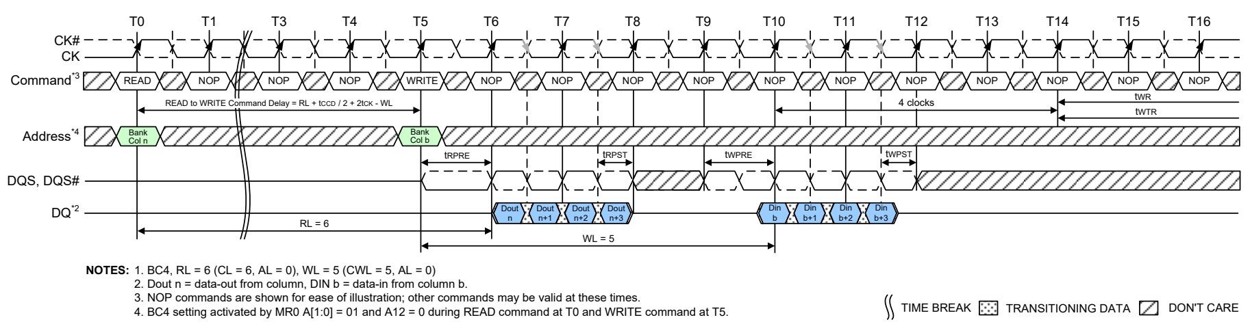
Figure 33 – READ (BC4) to WRITE (BC4) OTF
