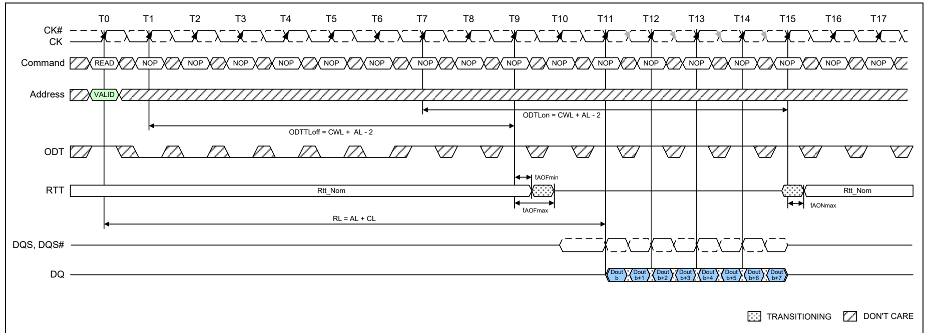
Figure 76 – ODT must be disabled externally during Reads by driving ODT low. (CL = 6; AL = CL - 1 = 5; RL = AL + CL = 11; CWL = 5; ODTLon = CWL + AL - 2 = 8; ODTLo = CWL + AL - 2 = 8)
