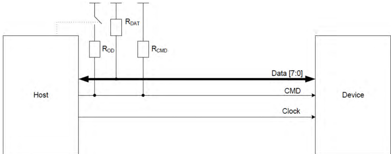
Figure 10: Bus Circuitry Diagram
