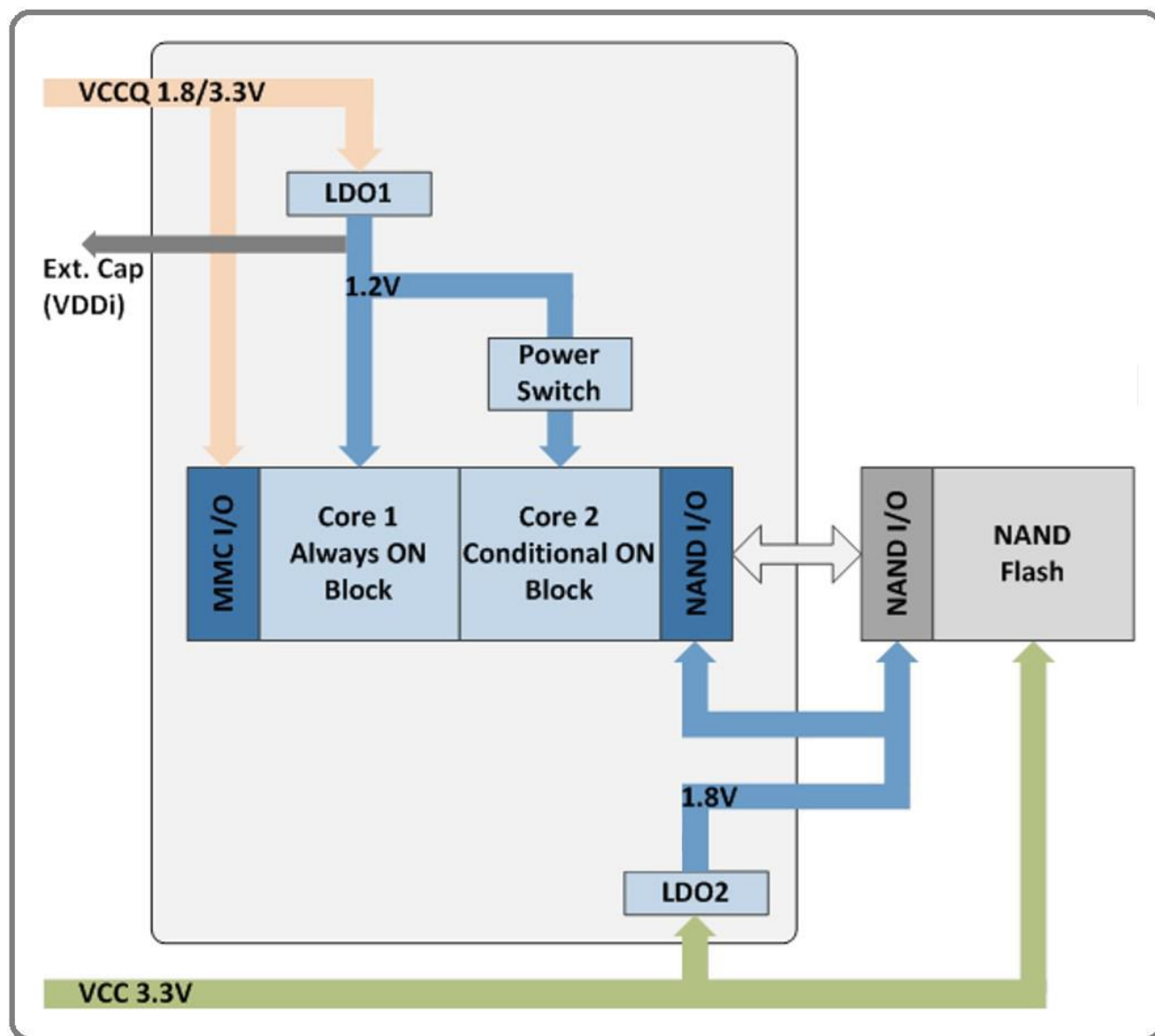
Figure 3. ASFC4G31M-51BIN Block Diagram
