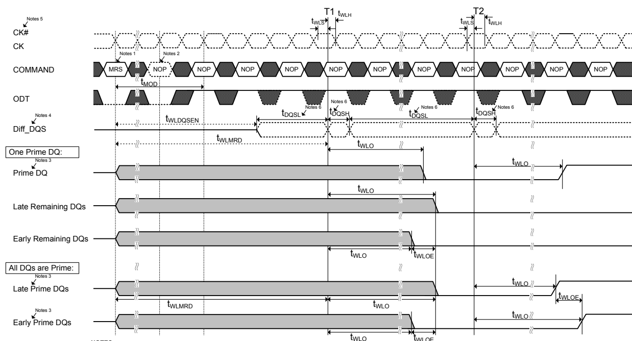
Figure 14. Timing details of Write Leveling sequence
