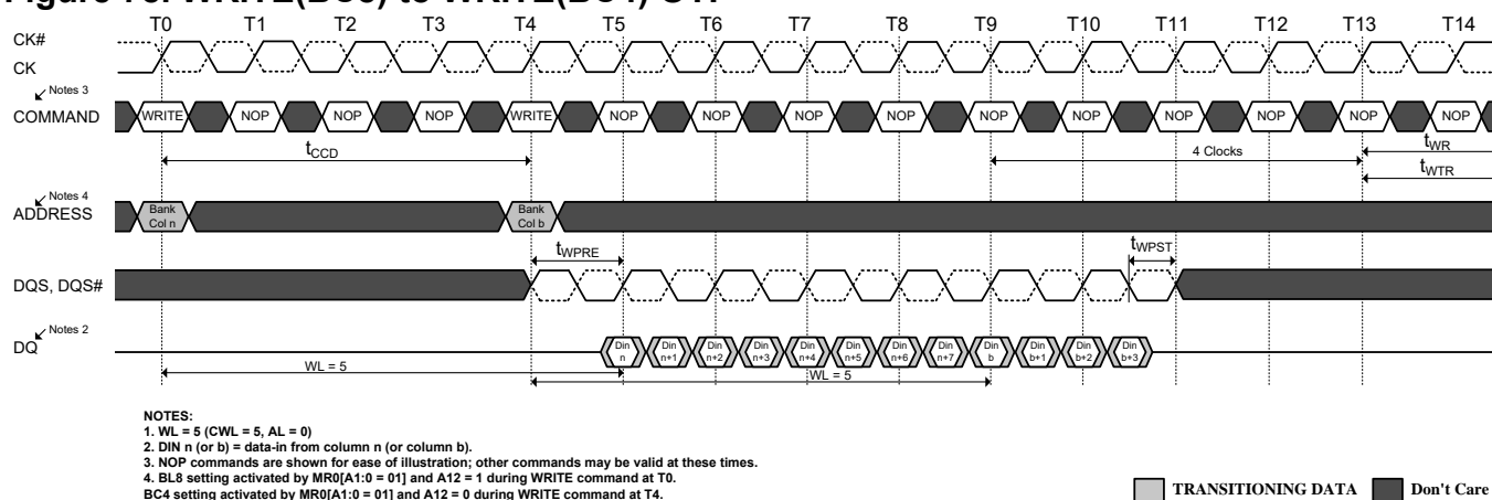
Figure 78. WRITE(BC8) to WRITE(BC4) OTF
