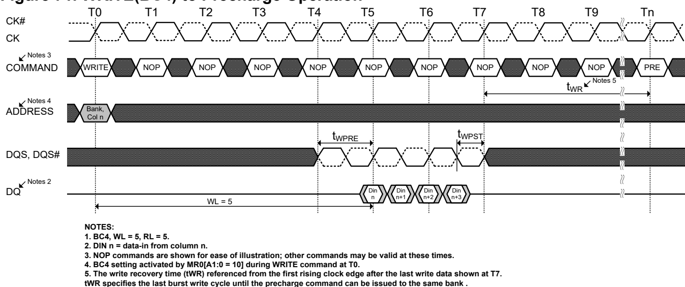
Figure 71. WRITE(BC4) to Precharge Operation
