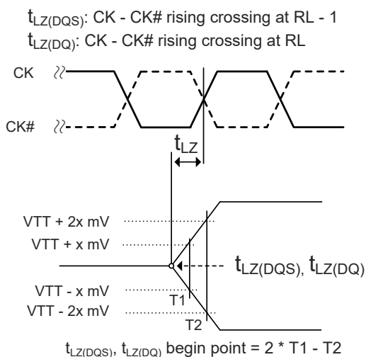
Figure 23. t_{LZ} and t_{HZ} method for calculating transitions and endpoints
