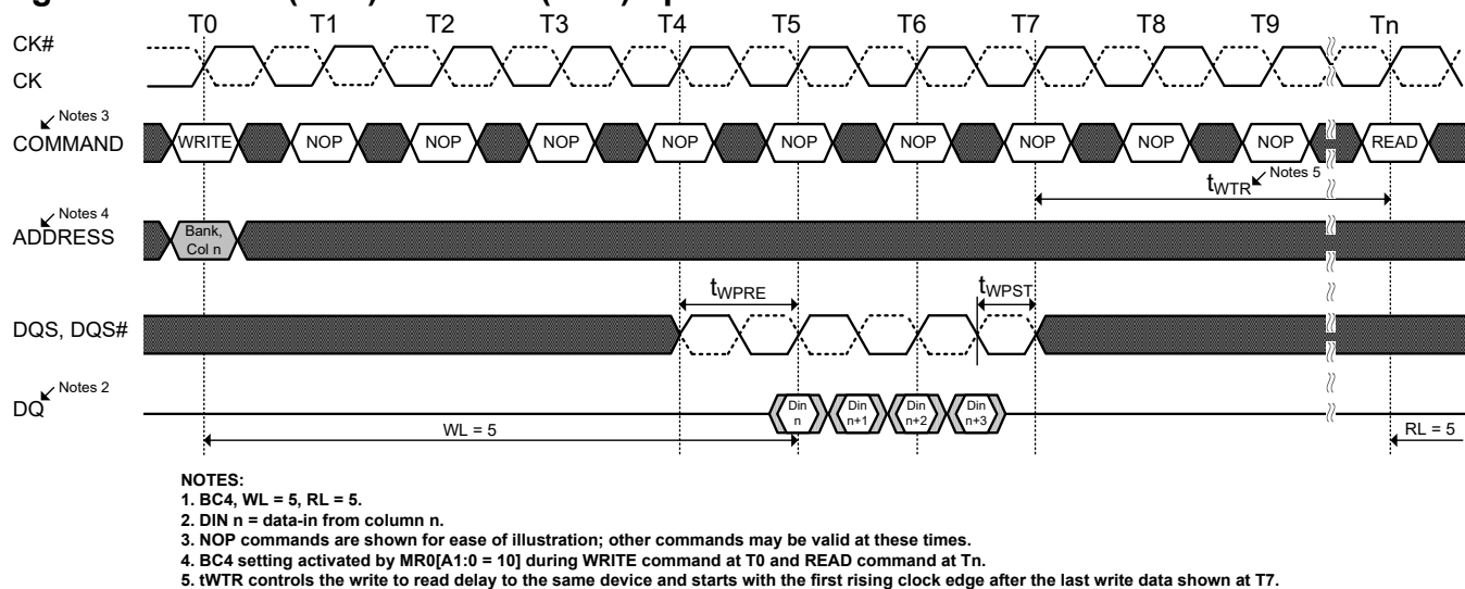
Figure 70. WRITE(BC4) to READ (BC4) operation
