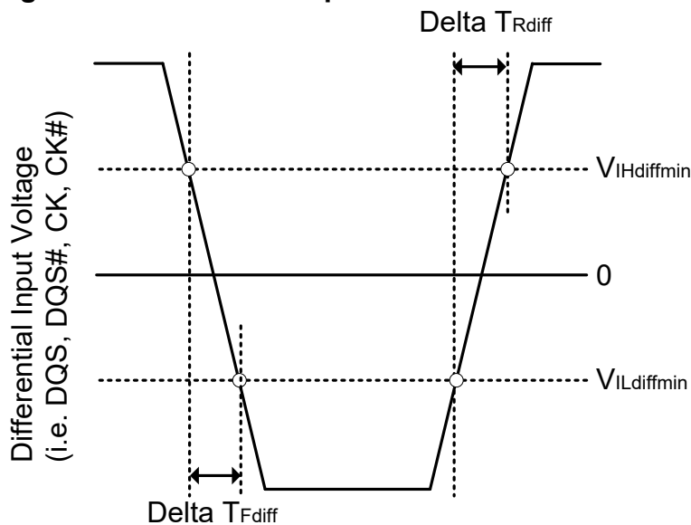
Figure 37. Differential Input Slew Rate Definition for DQS, DQS# and CK, CK#
