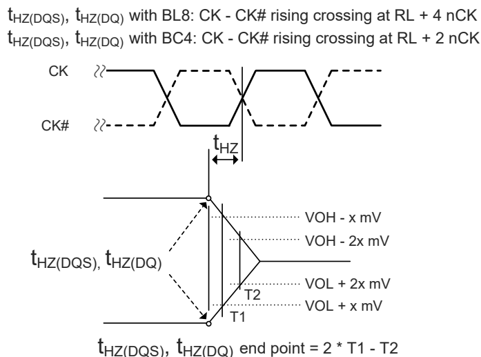
Figure 23. t_{LZ} and t_{HZ} method for calculating transitions and endpoints
