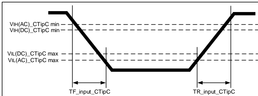
Figure 157 – Input C Slew Rate Definition
