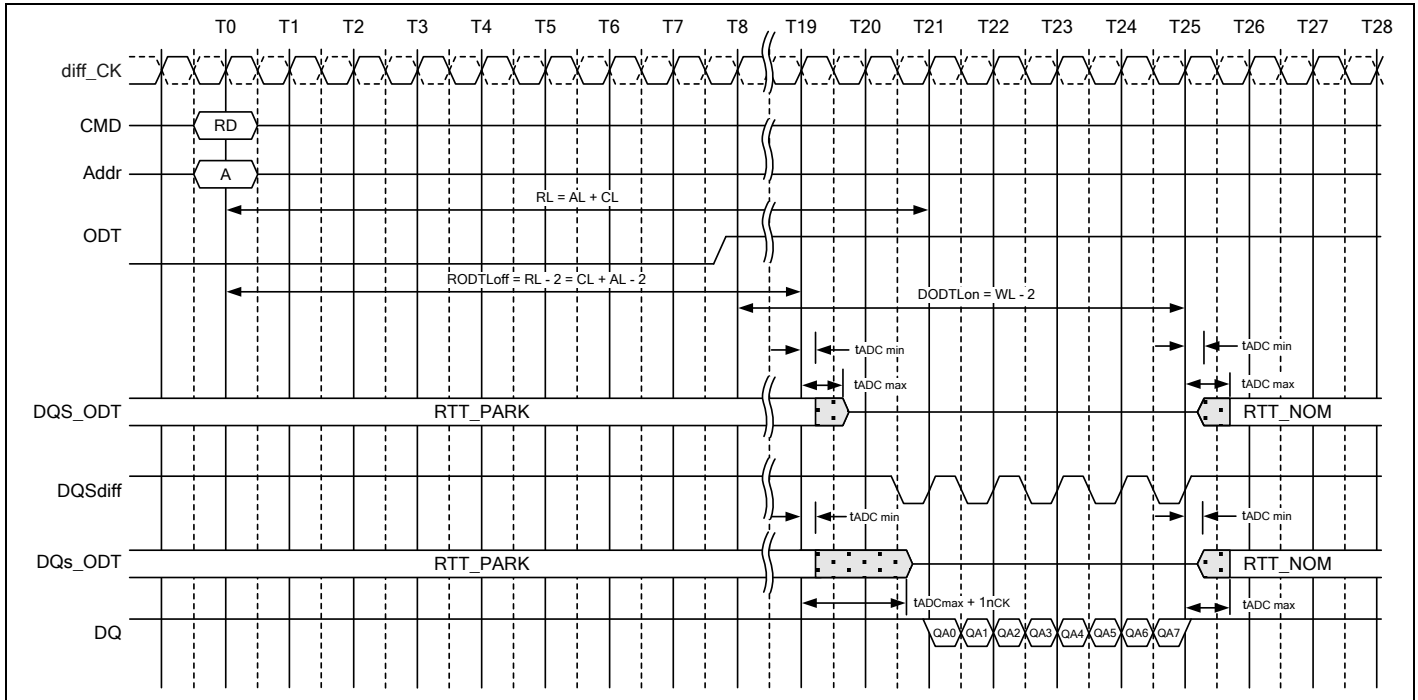
Figure 165 – Example: CL=11, PL=0; AL=CL-1=10; RL=AL+PL+CL=21; CWL=9; DODTLon=AL+CWL-2=17; RODTLoff=CL+AL-2=19; 1tCK preamble
