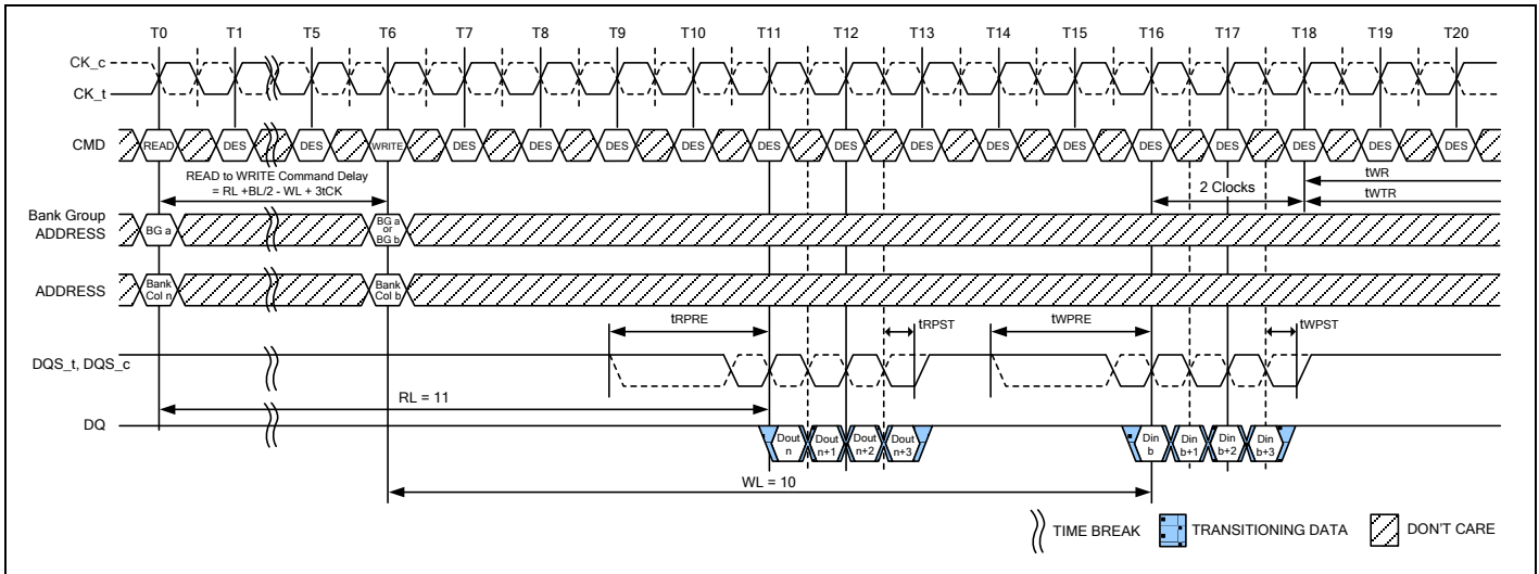
Figure 82 – READ (BC4) Fixed to WRITE (BC4) Fixed with 1tCK Preamble in Same or Different Bank Group
