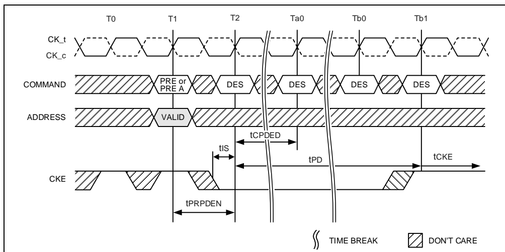
Figure 149 – Precharge/Precharge all Command to Power Down Entry
