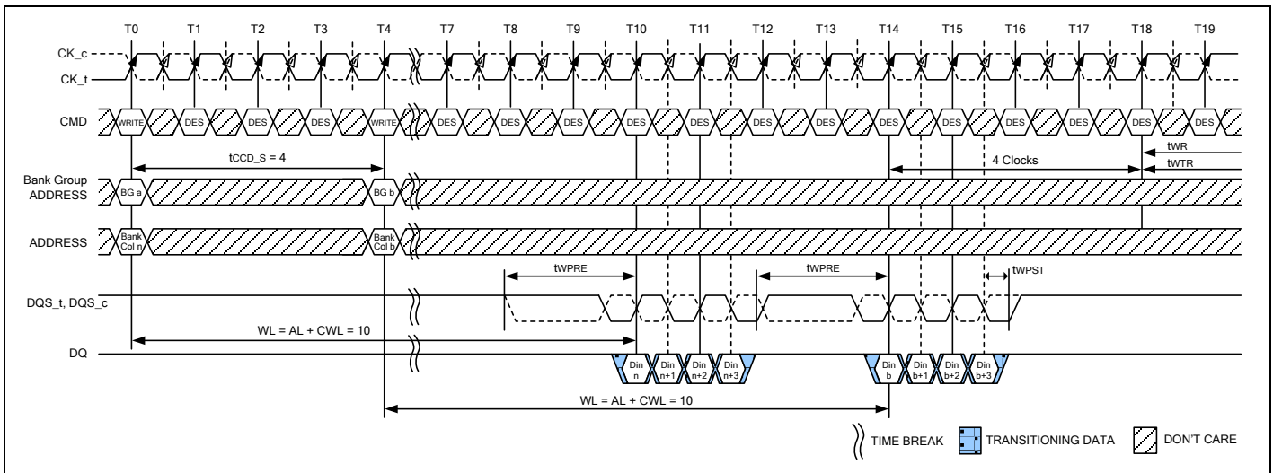
Figure 114 – WRITE (BC4) OTF to WRITE (BC4) OTF with 1tCK Preamble in Different Bank Group
