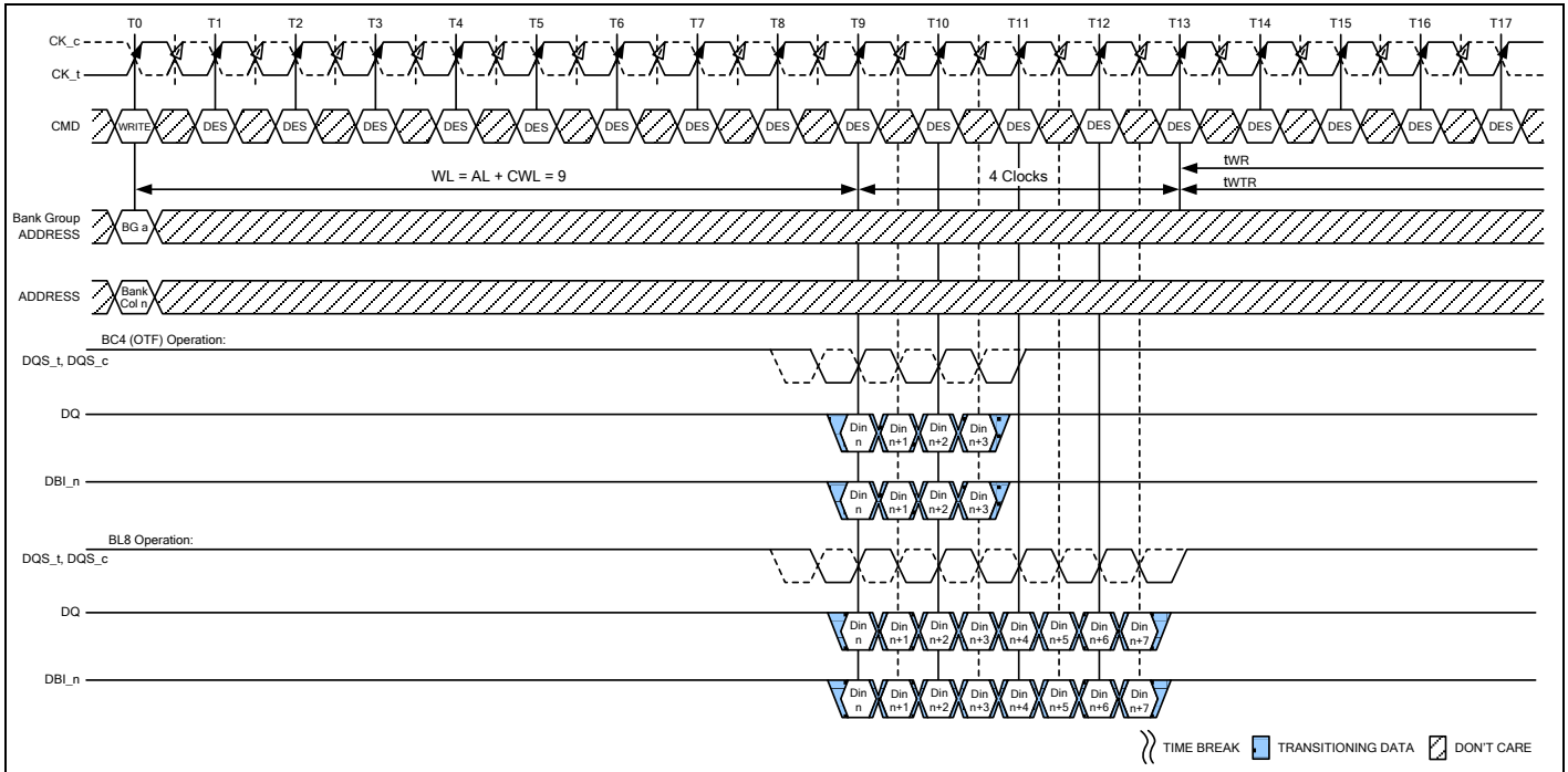
Figure 128 – WRITE (BC4) Fixed with Auto PRECHARGE Operation and 1tCK Preamble
