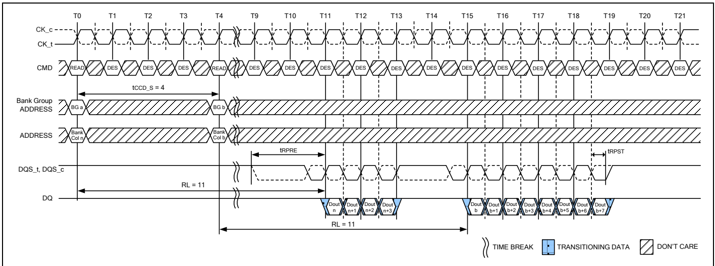
Figure 86 – READ (BC4) to READ (BL8) OTF with 1tCK Preamble in Different Bank Group
