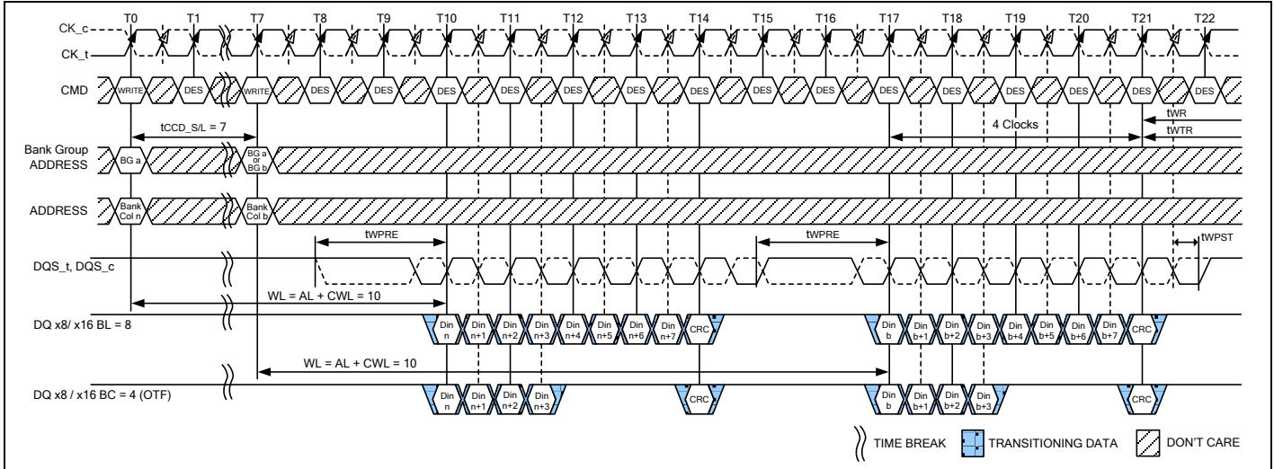
Figure 134 – Nonconsecutive WRITE (BL8/BC4 OTF) with 1tCK Preamble and Write CRC in Same or Different Bank Group
