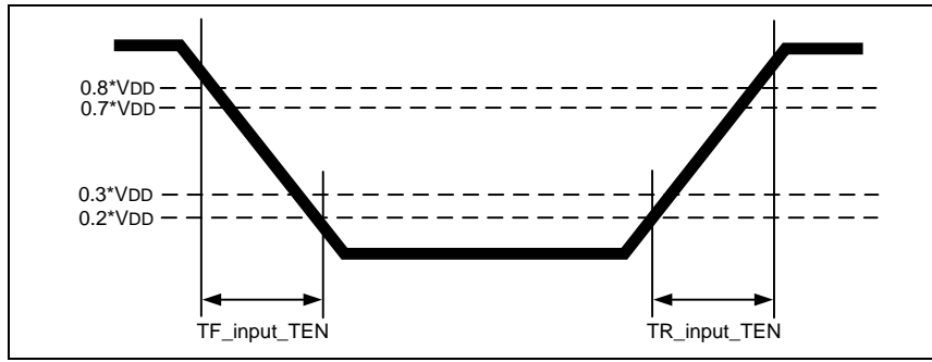
Figure 154 – TEN Input Slew Rate Definition
