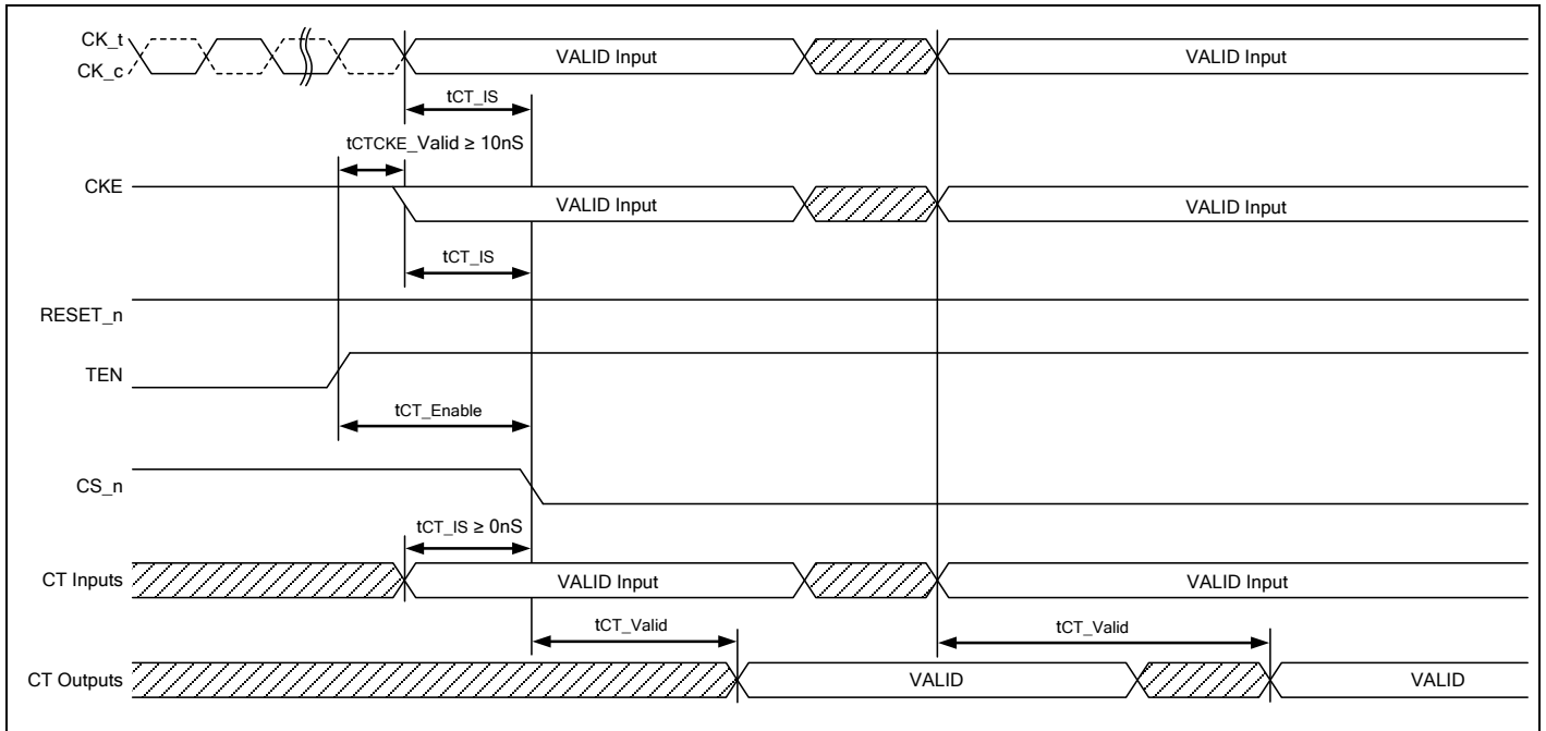
Figure 153 – Timing Diagram for Connectivity Test (CT) Mode
