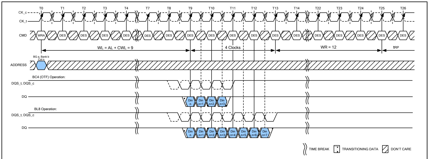
Figure 126 – WRITE (BC4) Fixed to PRECHARGE Operation with 1tCK Preamble
