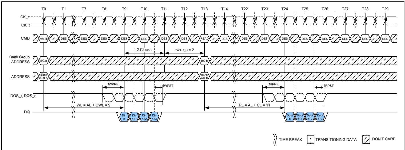
Figure 120 – WRITE (BC4) OTF to READ (BC4) OTF with 1tCK Preamble in Same Bank Group
