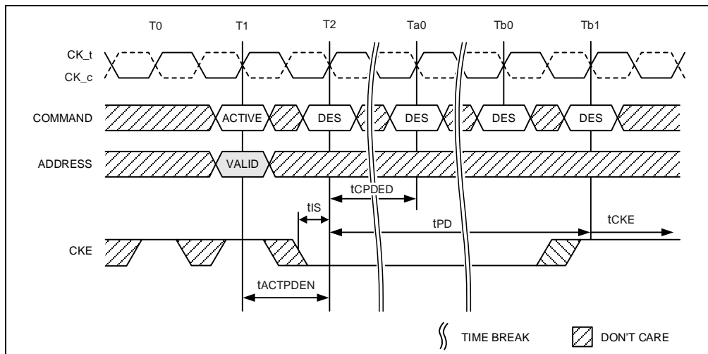
Figure 148 – Activate Command to Power Down Entry
