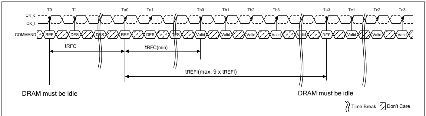
Figure 137 – Refresh Command Timing (Example of 1X Refresh mode)
