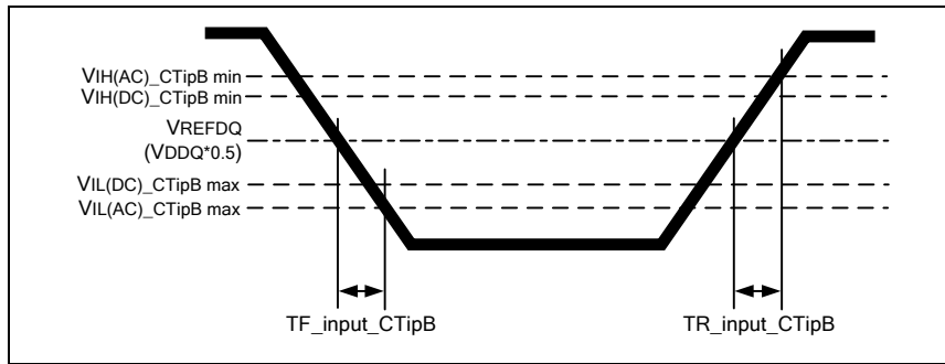
Figure 156 – Input B Slew Rate Definition
