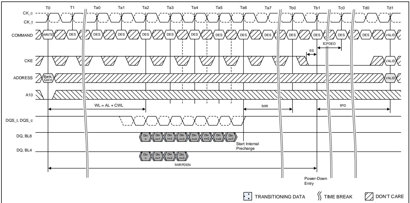
Figure 145 – Power Down Entry after Write
