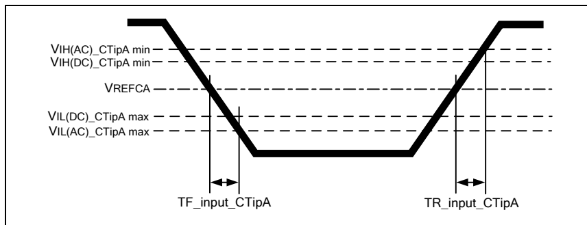
Figure 155 – CS_n and Input A Slew Rate Definition
