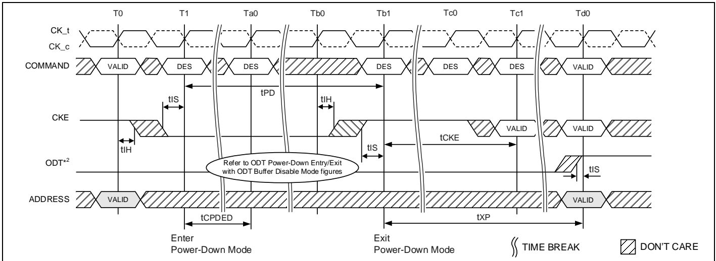
Figure 141 – Active Power Down Entry and Exit Timing Diagram MR5 bit A5 = 0
