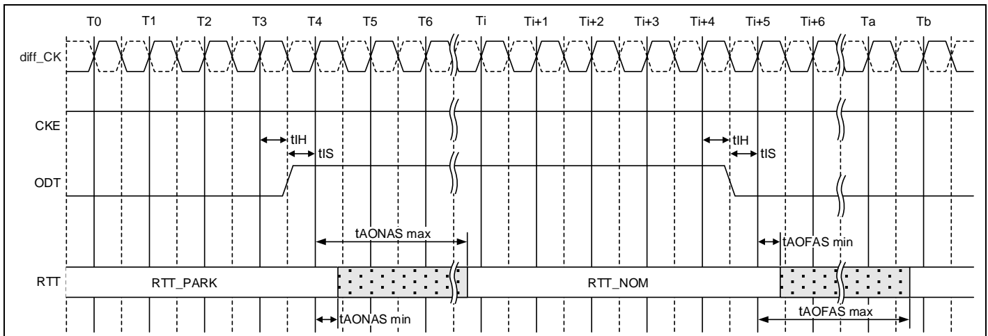
Figure 169 – Asynchronous ODT Timing on DDR4 SDRAM with DLL-off ODT Timing on DDR4 SDRAM with DLL-off
