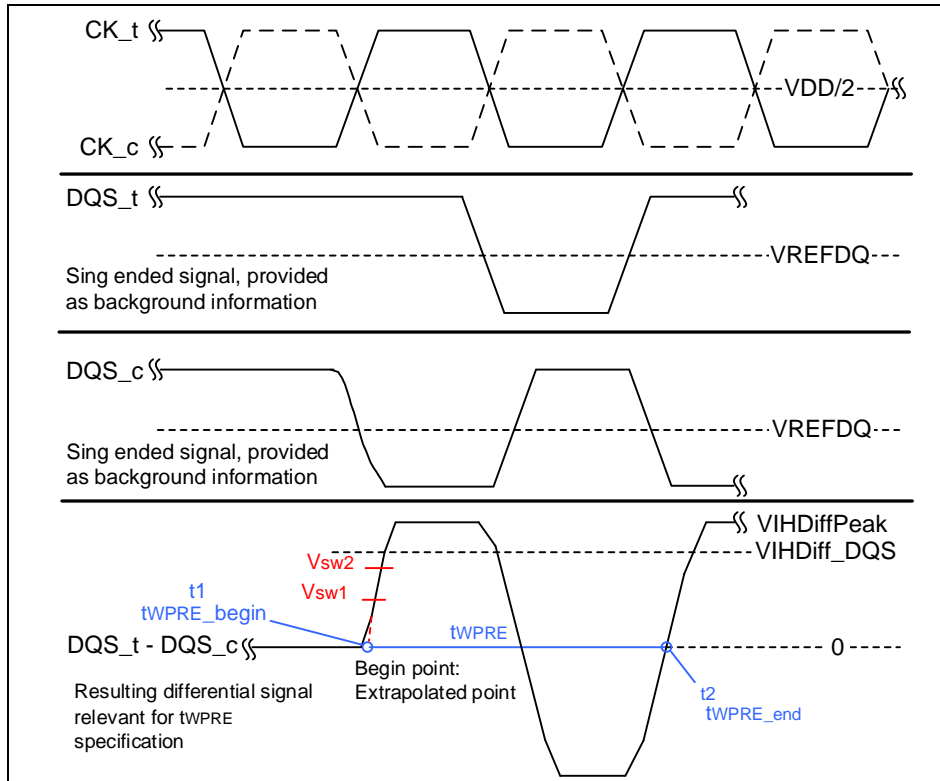
Figure 106 – Method for calculating tWPRE transitions and endpoints
