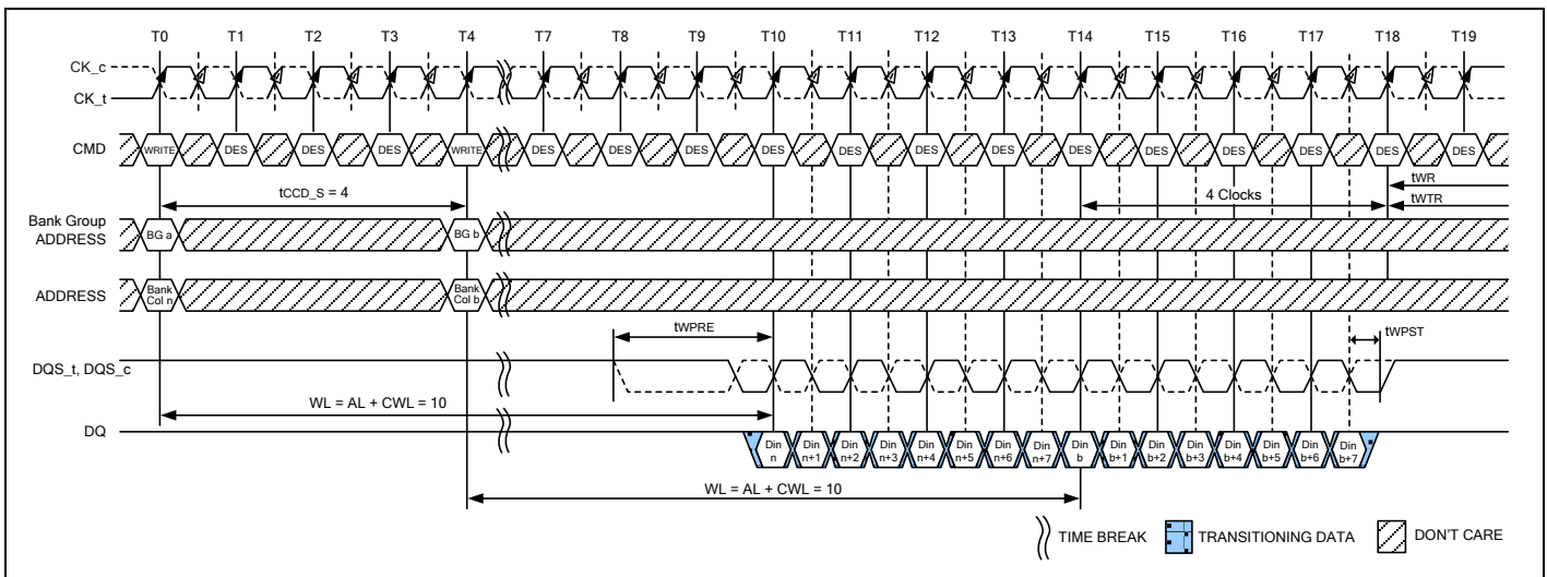
Figure 110 – Consecutive WRITE (BL8) with 1tCK Preamble in Different Bank Group
