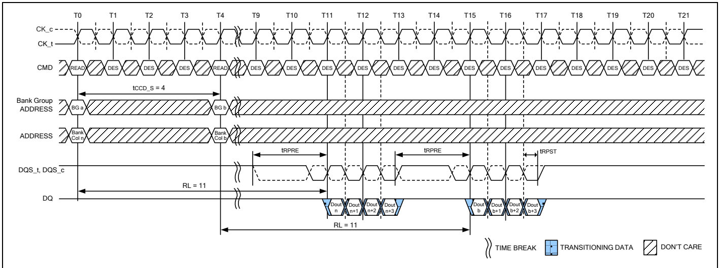
Figure 76 – READ (BC4) to READ (BC4) with 1tCK Preamble in Different Bank Group
