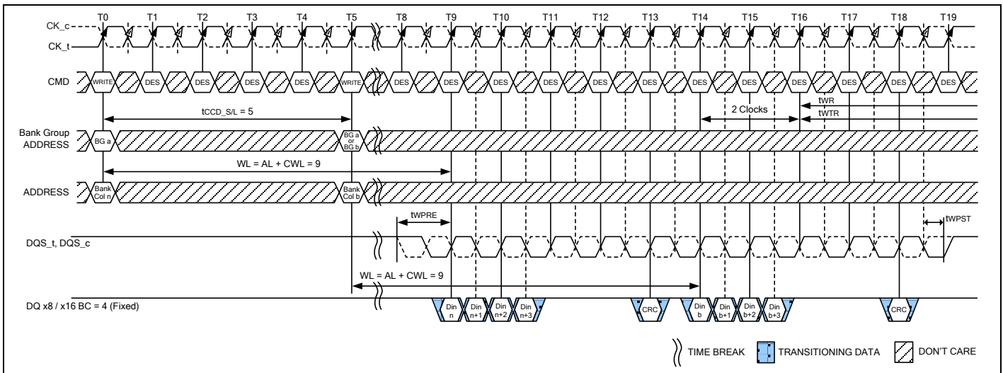
Figure 132 – Consecutive WRITE (BL8/BC4 OTF) with 1tCK Preamble and Write CRC in Same or Different Bank Group
