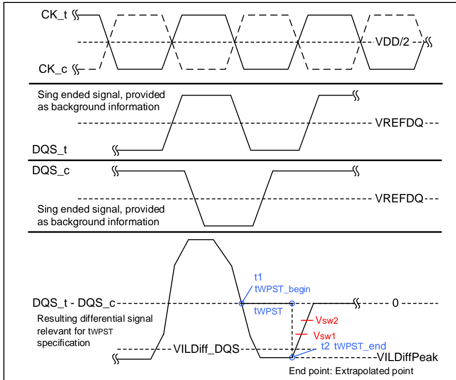
Figure 107 – Method for calculating tWPST transitions and endpoints
