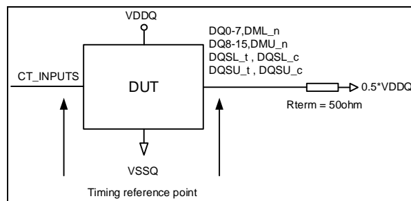
Figure 194 – Connectivity Test Mode Timing Reference Load
