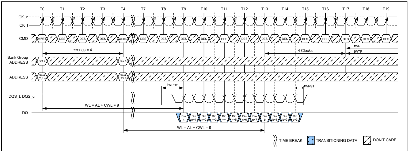
Figure 122 – WRITE (BC4) Fixed to READ (BC4) Fixed with 1tCK Preamble in Same Bank Group
