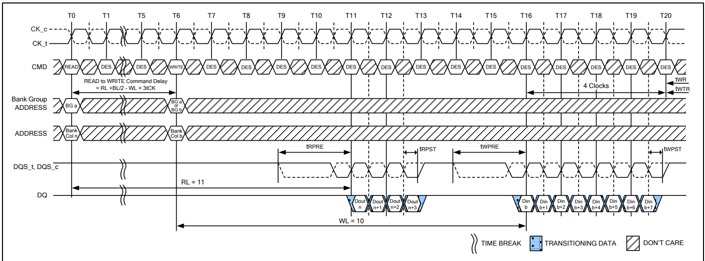
Figure 88 – READ (BC4) to WRITE (BL8) OTF with 1tCK Preamble in Same or Different Bank Group
