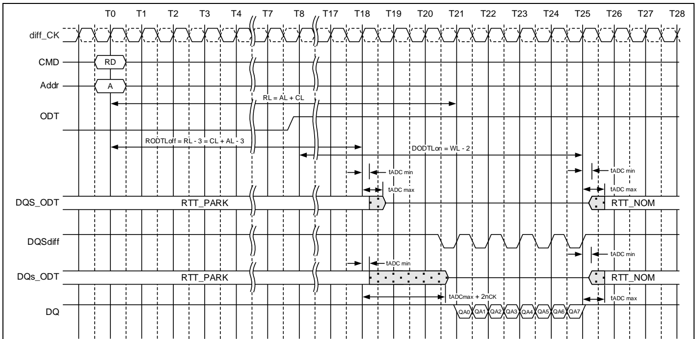
Figure 166 – Example: CL=11, PL=0; AL=CL-1=10; RL=AL+PL+CL=21; CWL=9; DODTLon=AL+CWL-2=17; RODTLoff=CL+AL-3=18; 2tCK preamble
