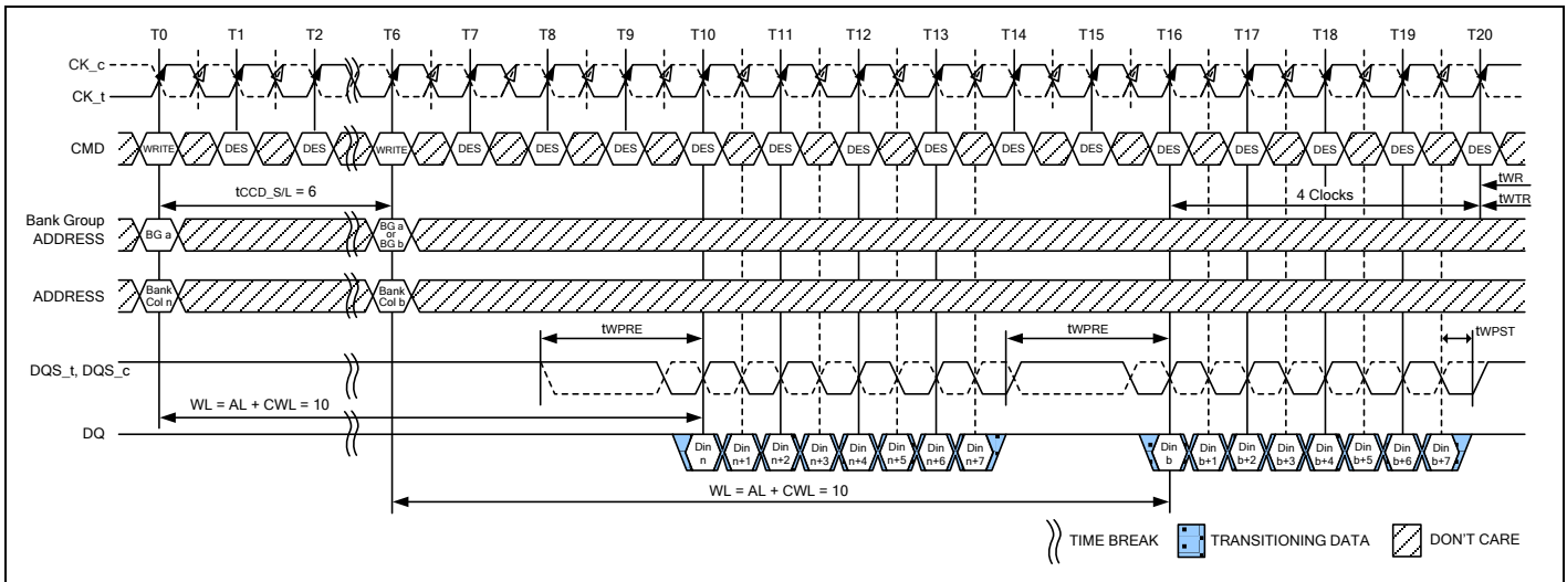
Figure 112 – Nonconsecutive WRITE (BL8) with 1tCK Preamble in Same or Different Bank Group
