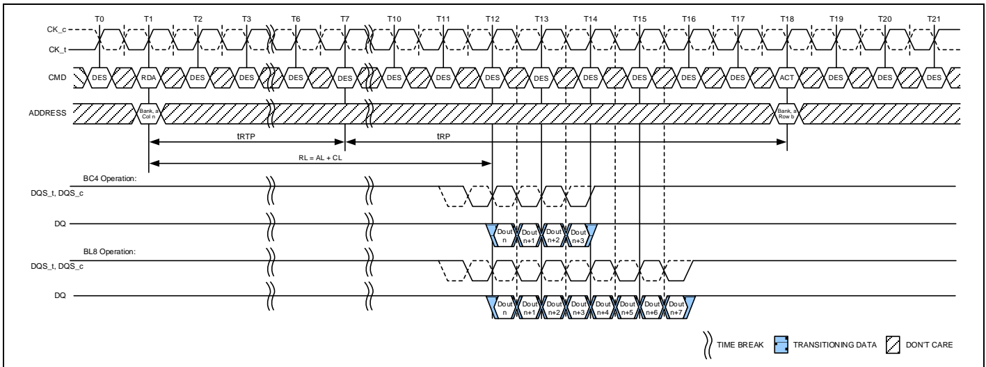
Figure 94 – READ to PRECHARGE with Additive Latency and 1tCK Preamble
