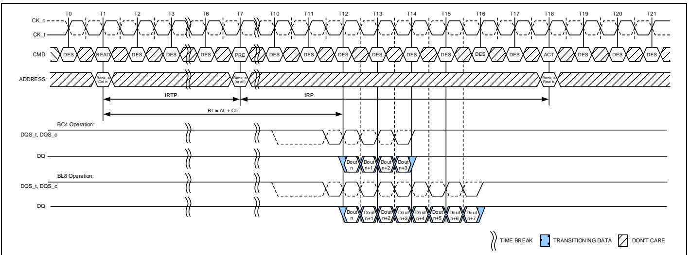
Figure 92 – READ to PRECHARGE with 1tCK Preamble
