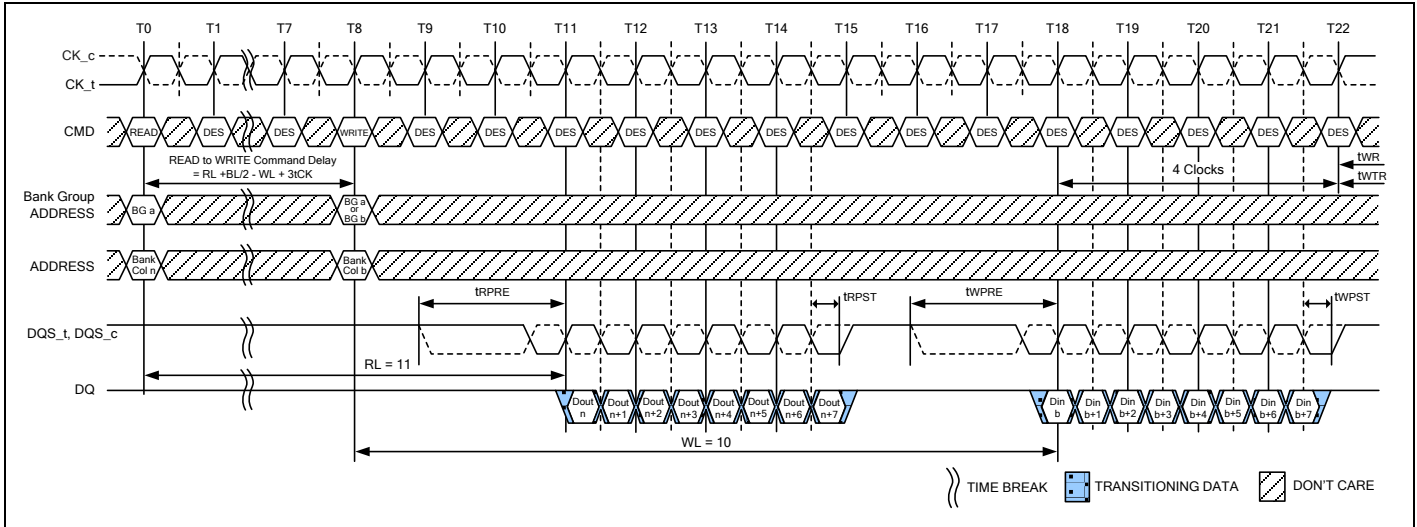
Figure 78 – READ (BL8) to WRITE (BL8) with 1tCK Preamble in Same or Different Bank Group
