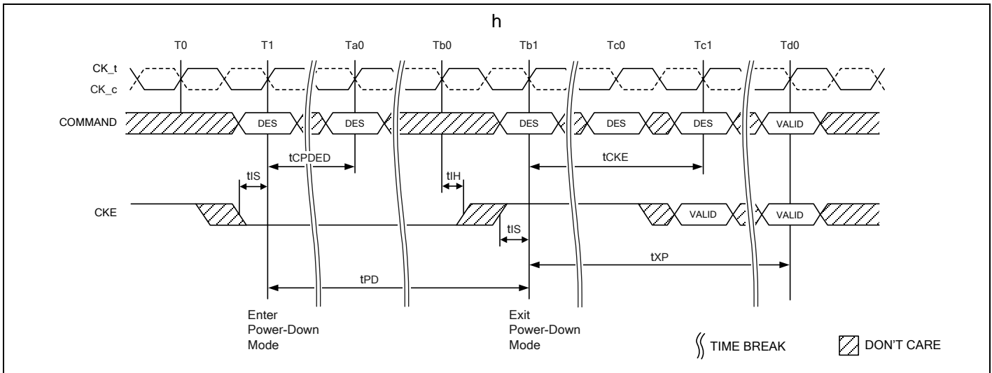
Figure 146 – Precharge Power Down Entry and Exit
