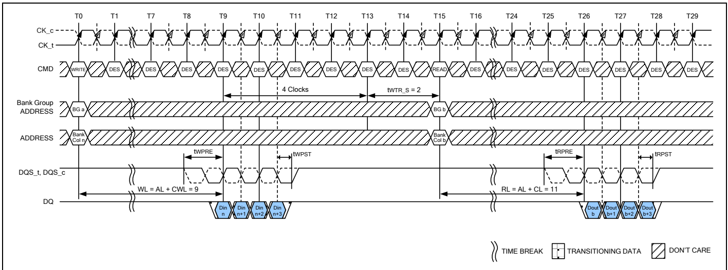
Figure 118 – WRITE (BL8) to READ (BL8) with 1tCK Preamble in Same Bank Group
