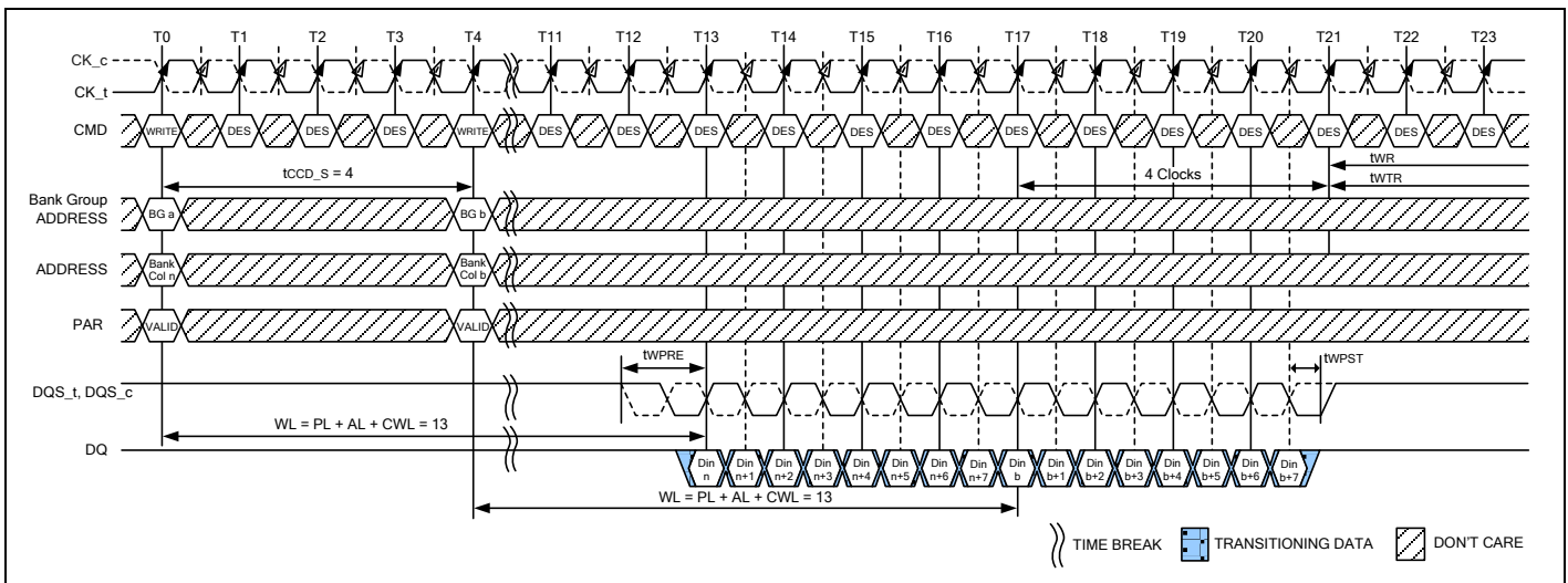
Figure 130 – WRITE (BC4) Fixed with 1tCK Preamble and DBI
