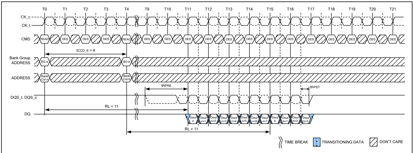
Figure 84 – READ (BL8) to READ (BC4) OTF with 1tCK Preamble in Different Bank Group
