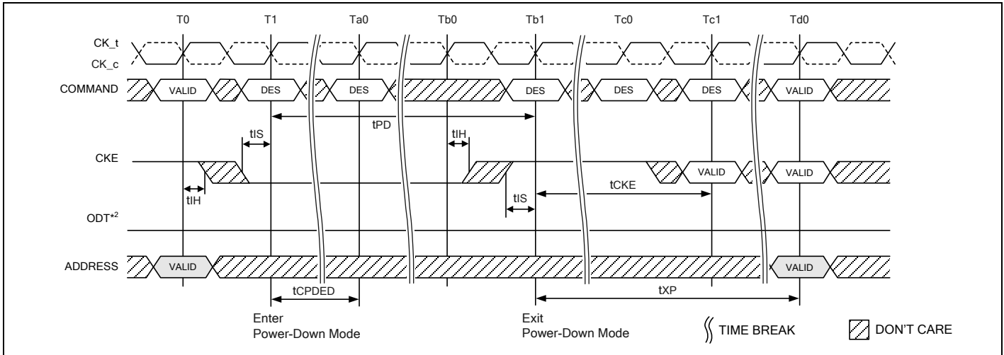
Figure 141 – Active Power Down Entry and Exit Timing Diagram MR5 bit A5 = 0
