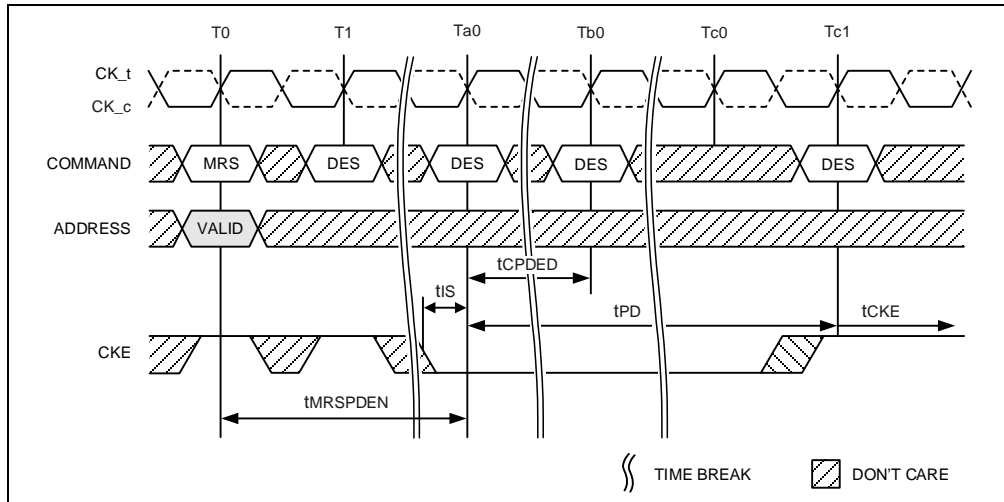
Figure 150 – MRS Command to Power Down Entry
