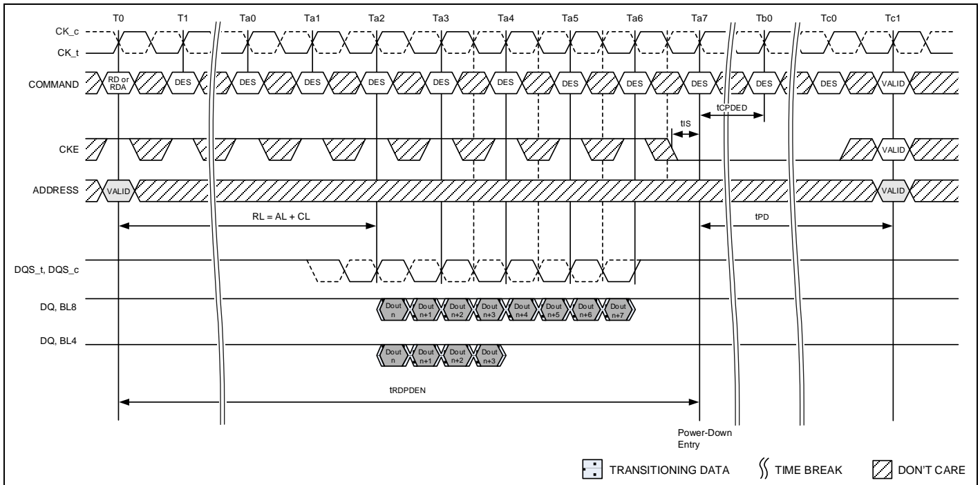
Figure 143 – Power Down Entry after Read or Read with Auto Precharge
