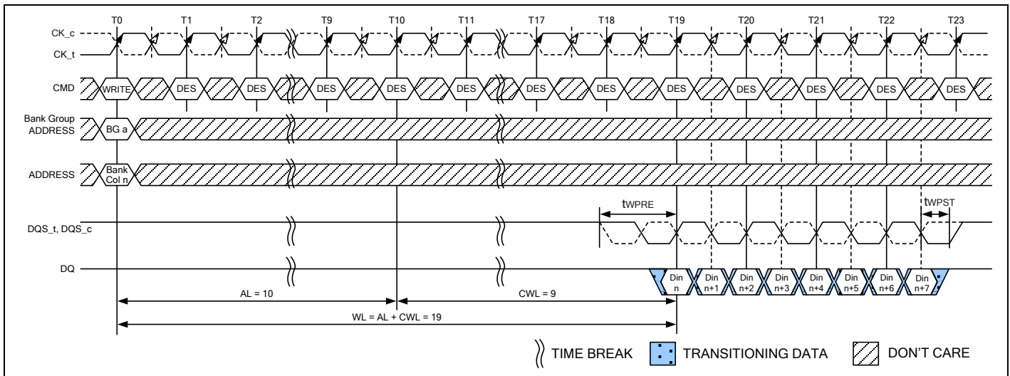
Figure 108 – WRITE Burst Operation WL = 9 (AL = 0, CWL = 9, BL8)
