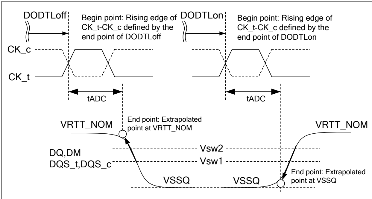
Figure 173 – Definition of t ADC at Direct ODT Control
