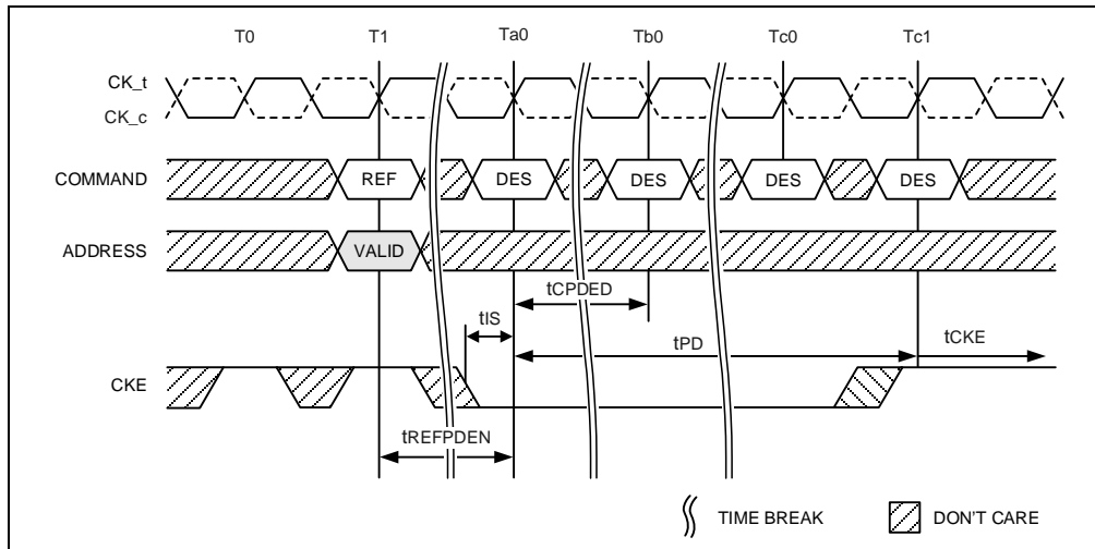
Figure 147 – Refresh Command to Power Down Entry
