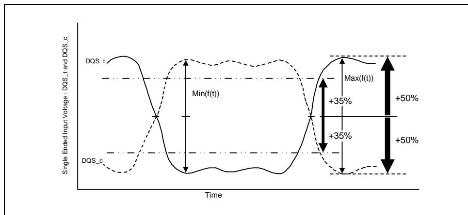
Figure 187 – Definition of differential DQS Peak Voltage and rage of exempt non-monotonic signaling
