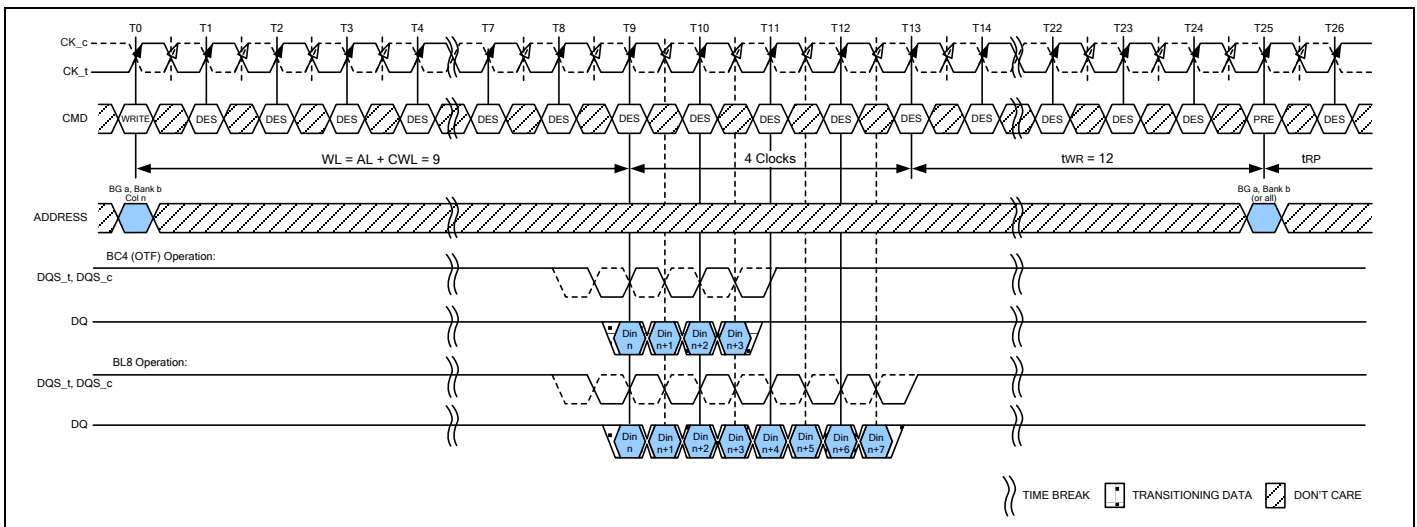
Figure 124 – WRITE (BC4) OTF to WRITE (BL8) with 1tCK Preamble in Different Bank Group
