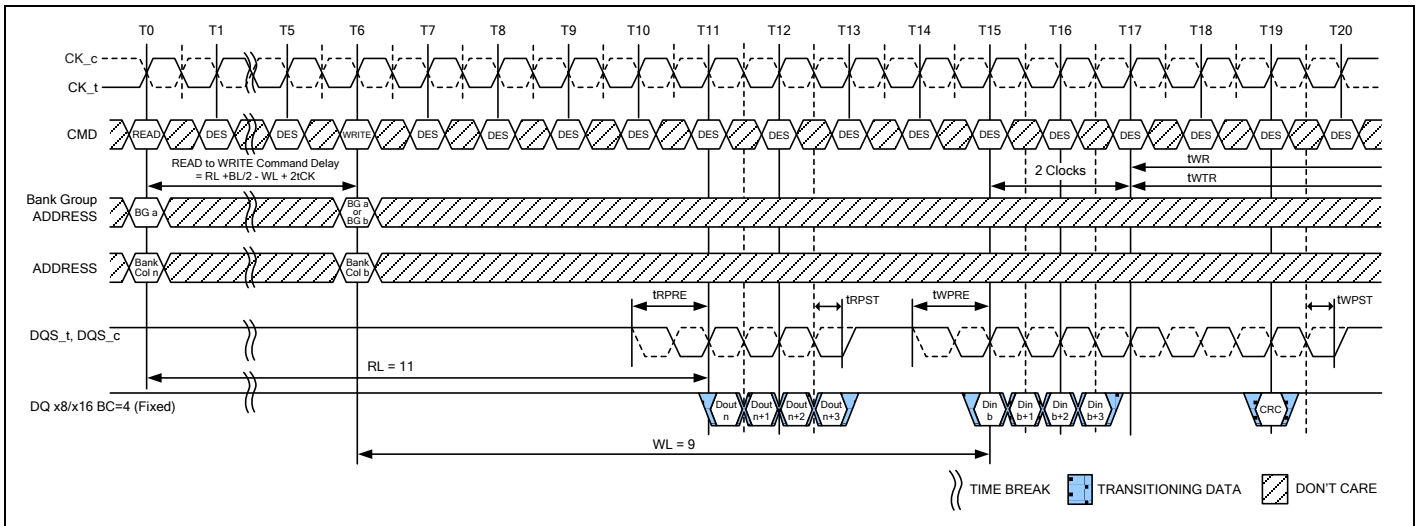
Figure 100 – READ (BL8) to WRITE (BL8 or BC4: OTF) with 1tCK Preamble and Write CRC in Same or Different Bank Group
