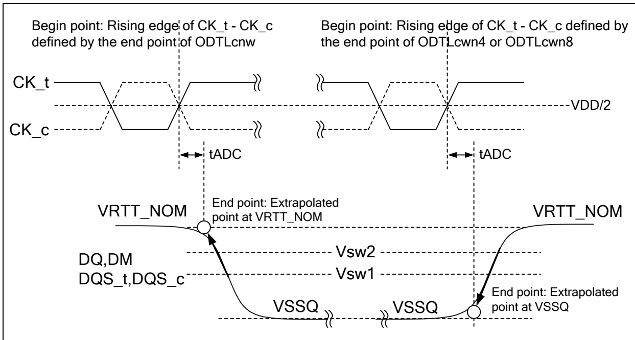
Figure 174 – Definition of t ADC at Dynamic ODT Control
