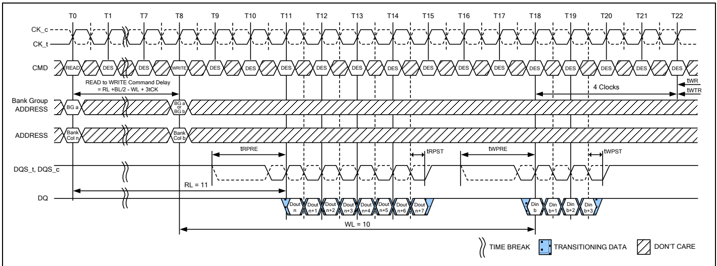
Figure 90 – READ (BL8) to WRITE (BC4) OTF with 1tCK Preamble in Same or Different Bank Group
