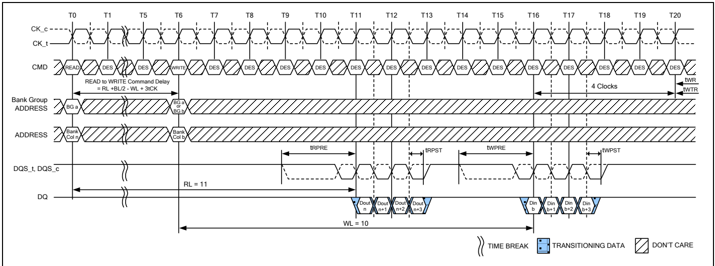
Figure 80 – READ (BC4) OTF to WRITE (BC4) OTF with 1tCK Preamble in Same or Different Bank Group
