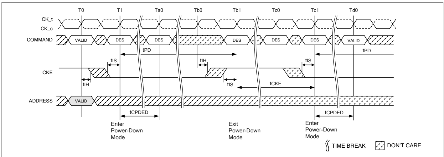
Figure 151 – Power Down Entry/Exit Clarification
