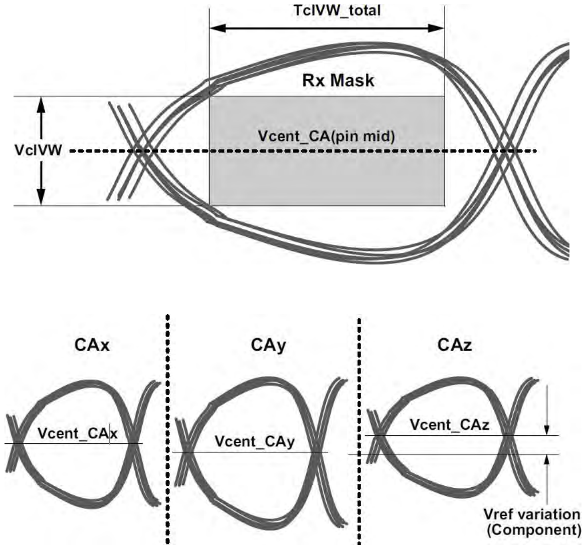
Figure 27. Across pin V_{REFCA} voltage variation
