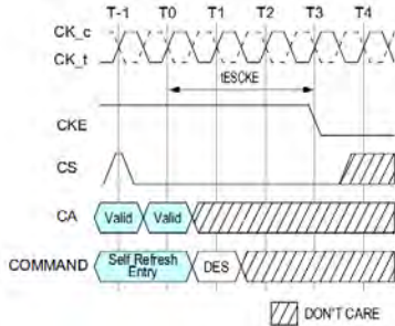
Figure 23. tESCKE Timing
