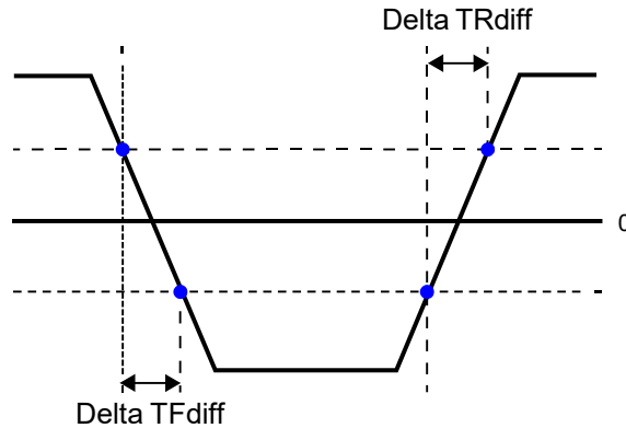
Figure 17. Differential Output Slew Rate Definition
