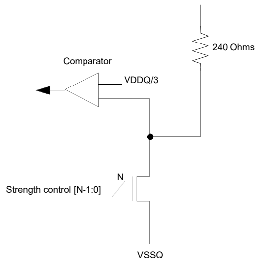
Figure 21. pull-down calibration
