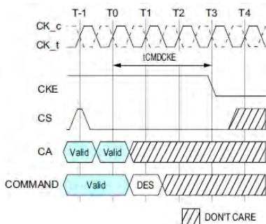
Figure 24. tCMDCKE Timing
