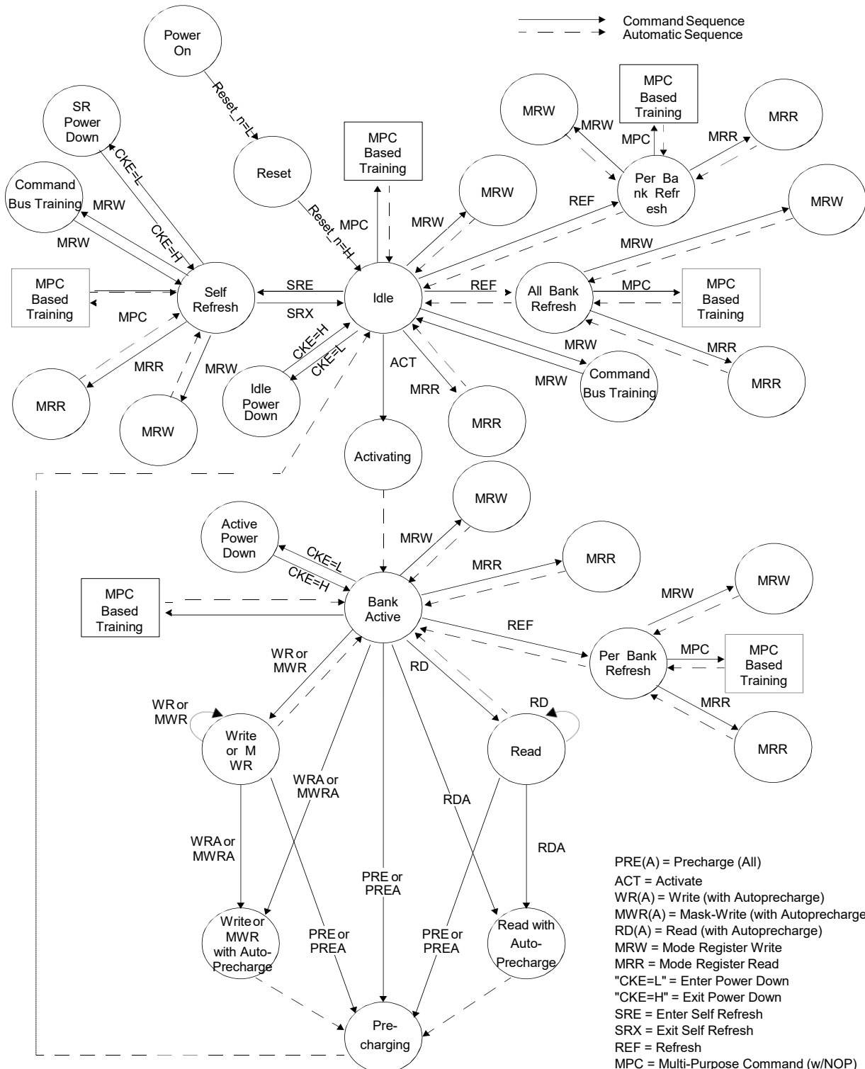
Figure 1. LPDDR4X: Simplified Bus Interface State Diagram-1
