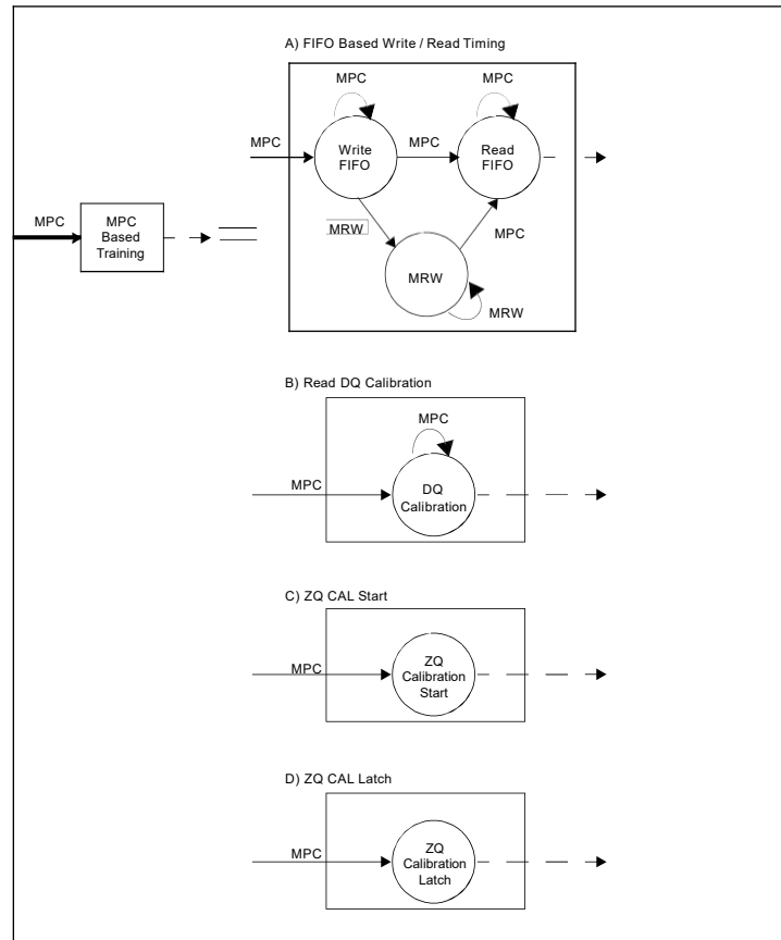
Figure 2. LPDDR4X: Simplified Bus Interface State Diagram -2
