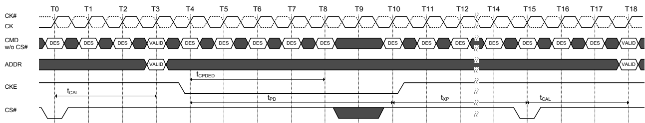
Figure 21. Self Refresh Entry/Exit Timing with CAL
