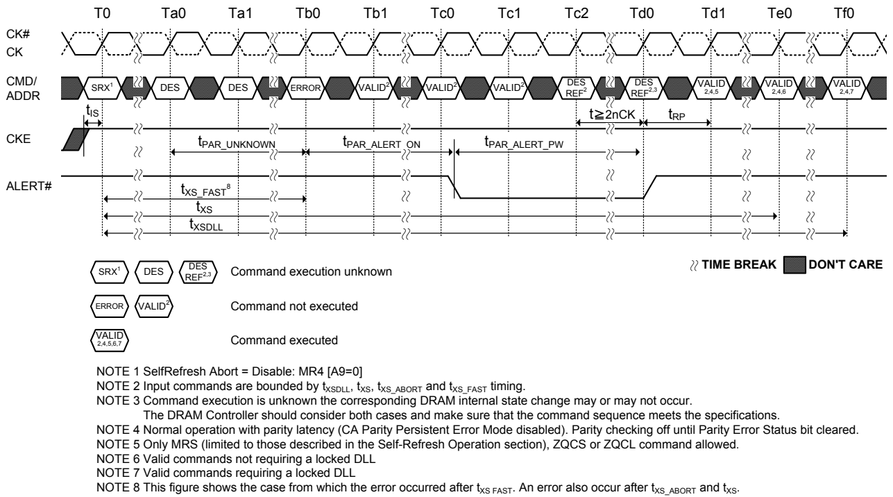
Figure 61. CA Parity Error Checking - SRX
