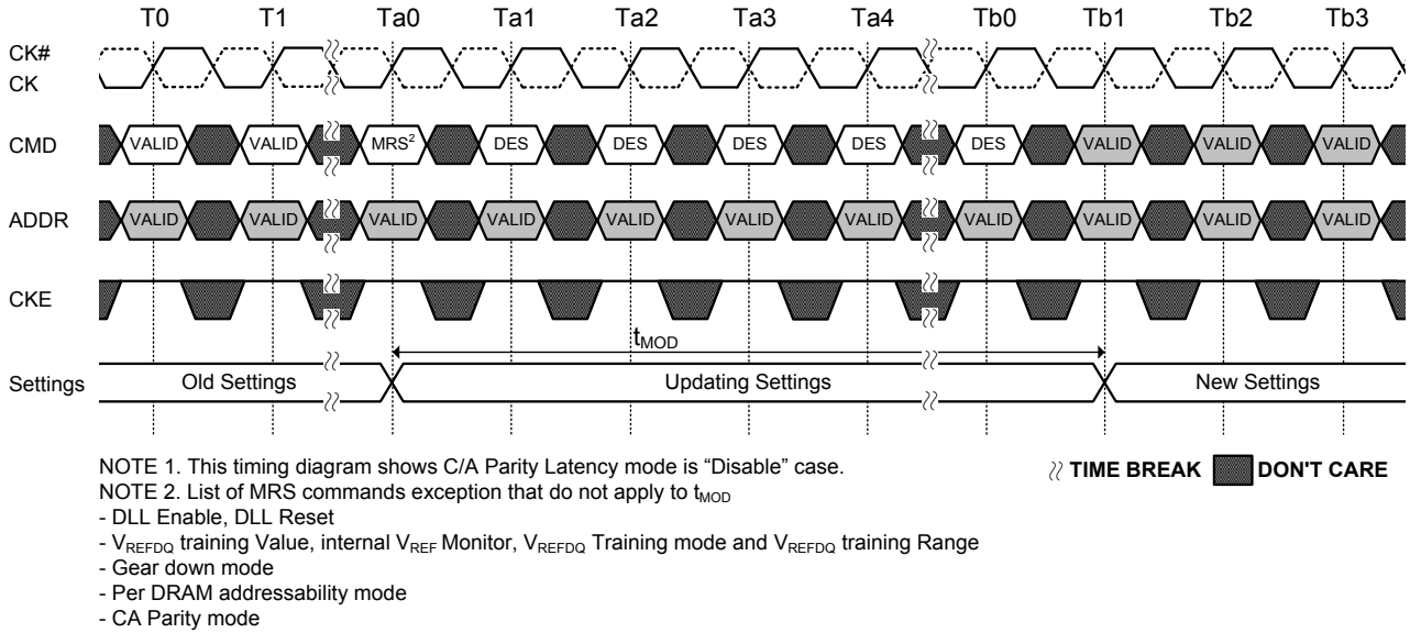
Figure 7. t_{MOD} timing
