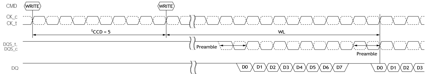
Figure 106: 1^t\text{CK} vs. 2^t\text{CK} WRITE Preamble Mode, t_{\text{CCD}} = 5
