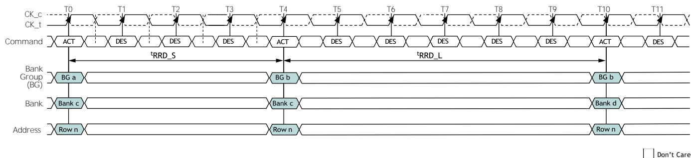
Figure 115: t_{RRD} Timing
