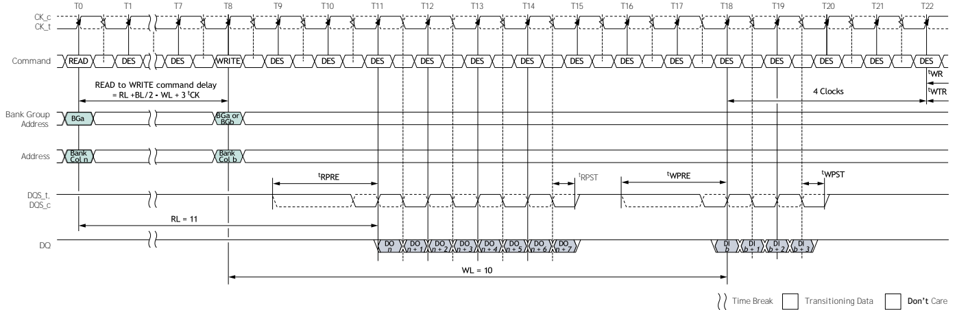
Figure 145: READ (BL8) to WRITE (BC4) OTF with 2 t CK Preamble in Same or Different Bank Group
