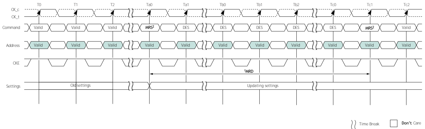
Figure 11: t_{MRD} Timing
