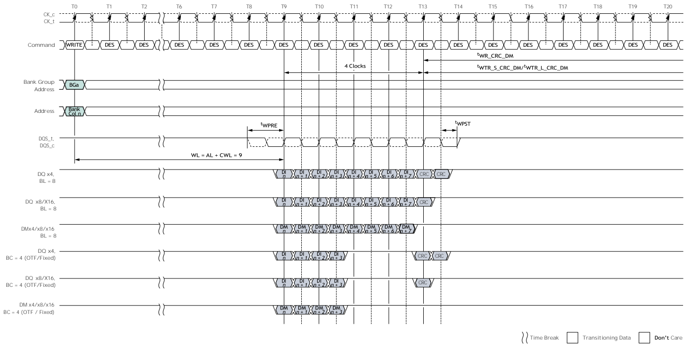
Figure 194: WRITE (BL8/BC4-OTF/Fixed) with t^1\text{CK} Preamble and Write CRC in Same or Different Bank Group
