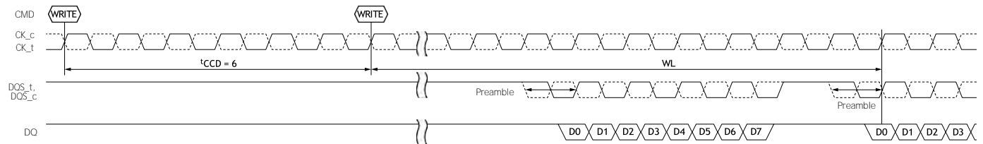
Figure 107: 1^t\text{CK} vs. 2^t\text{CK} WRITE Preamble Mode, t_{\text{CCD}} = 6
