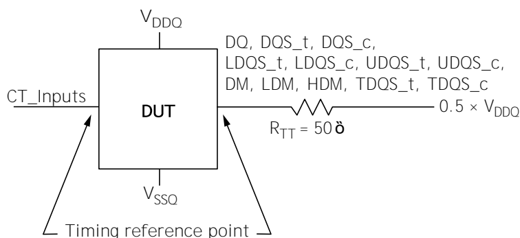
Figure 229: Connectivity Test Mode Output Slew Rate Definition
