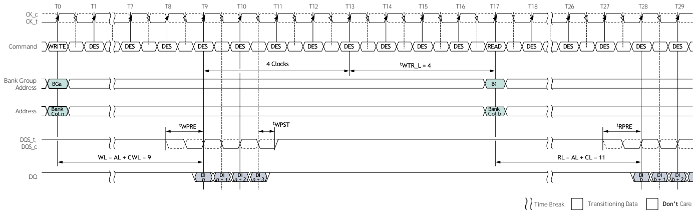
Figure 180: WRITE (BC4) OTF to READ (BC4) OTF with 1^t\text{CK} Preamble in Same Bank Group
