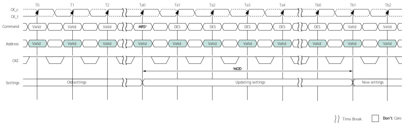
Figure 12: t_{MOD} Timing
