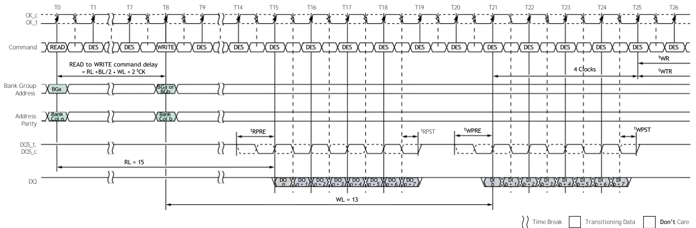
Figure 153: READ (BL8) to WRITE (BL8) with 1^t\text{CK} Preamble and CA Parity in Same or Different Bank Group
