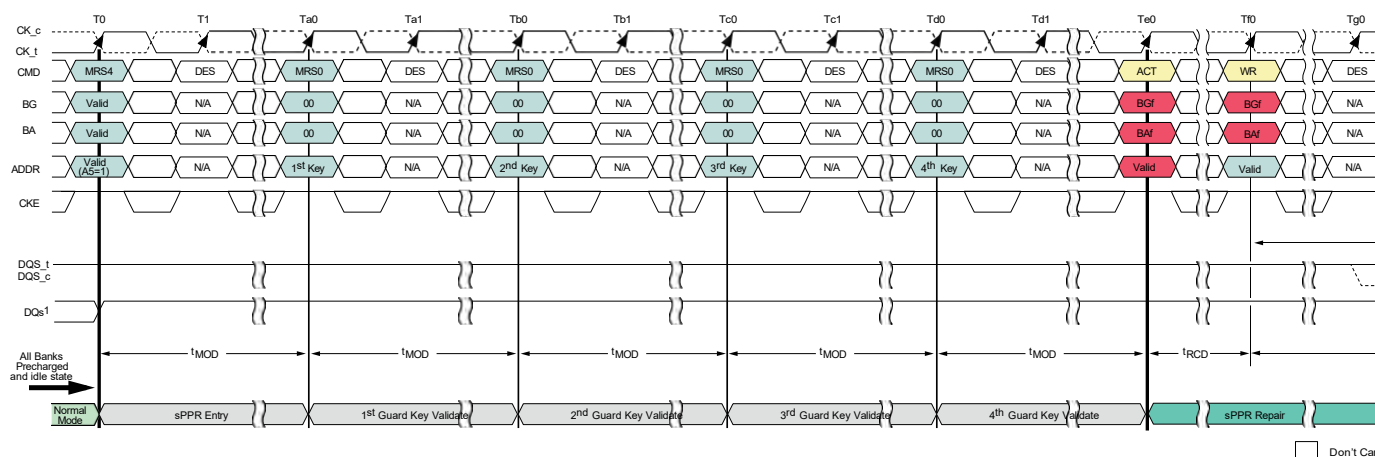
Figure 73: sPPR - Entry
