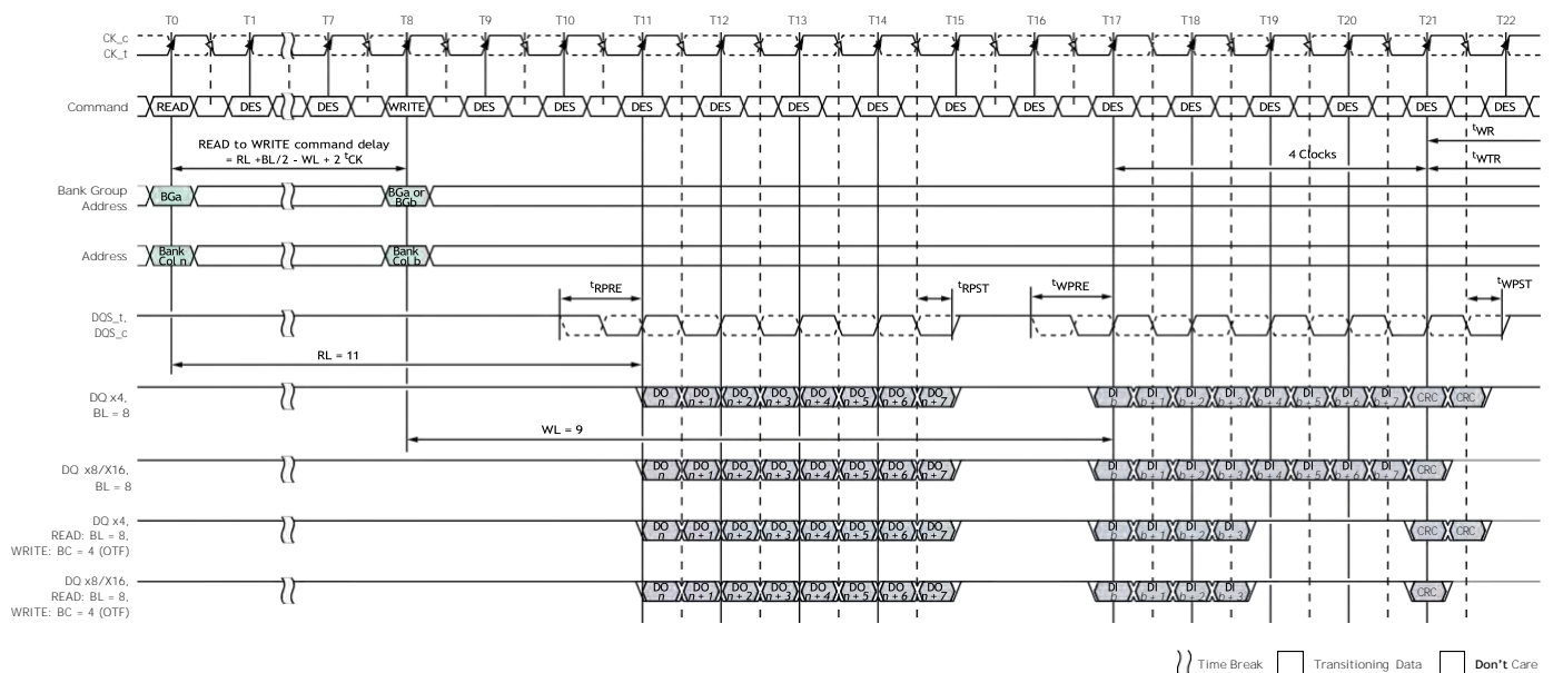
Figure 154: READ (BL8) to WRITE (BL8 or BC4: OTF) with 1^t\text{CK} Preamble and Write CRC in Same or Different Bank Group
