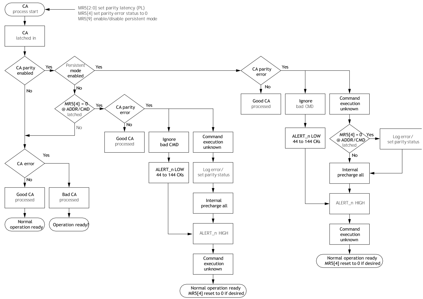
Figure 55: CA Parity Flow Diagram
