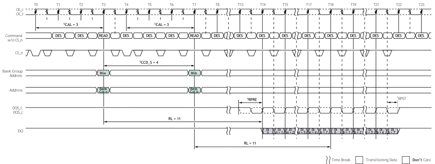
Figure 156: Consecutive READ (BL8) with CAL ( 3^t\text{CK} ) and 1^t\text{CK} Preamble in Different Bank Group
