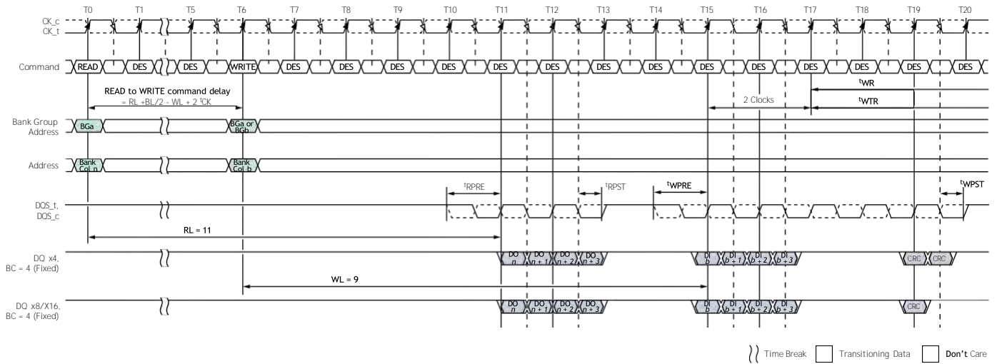
Figure 155: READ (BC4: Fixed) to WRITE (BC4: Fixed) with 1^t\text{CK} Preamble and Write CRC in Same or Different Bank Group
