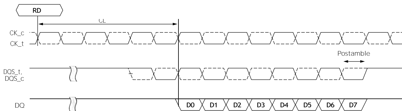
Figure 111: READ Postamble
