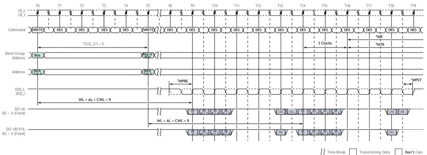
Figure 191: Consecutive WRITE (BC4-Fixed) with 1^t\text{CK} Preamble and Write CRC in Same or Different Bank Group
