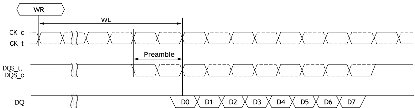
Figure 104: 1^t\text{CK} vs. 2^t\text{CK} WRITE Preamble Mode
