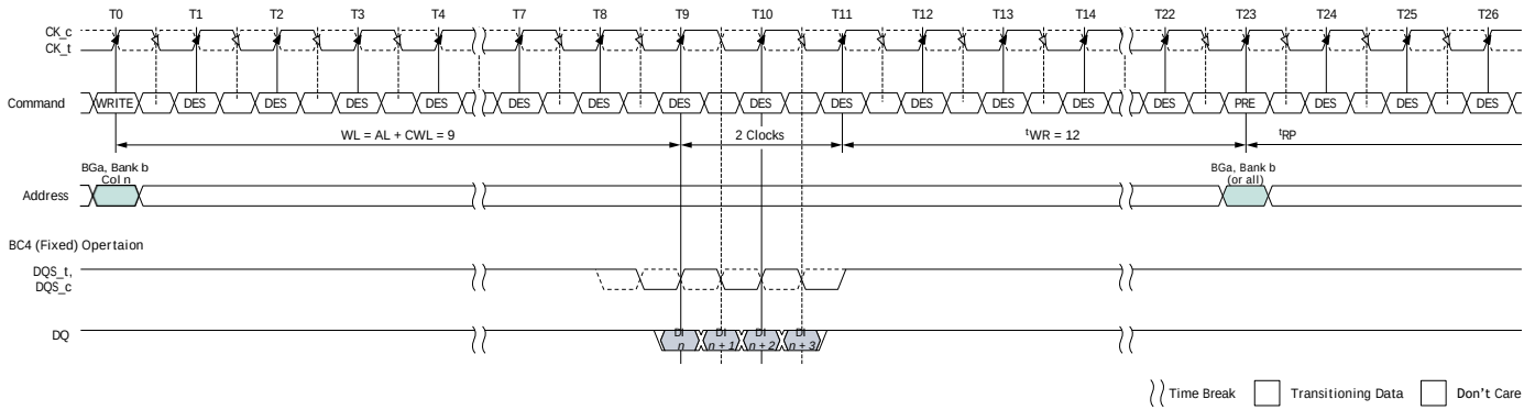
Figure 184: WRITE (BC4-Fixed) to PRECHARGE with 1t_{CK} Preamble
