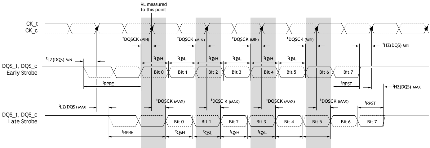
Figure 119: Clock-to-Data Strobe Relationship
