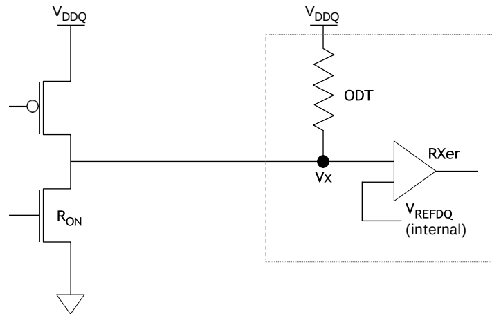
Figure 67: V_{\text{REFDQ}} Equivalent Circuit
