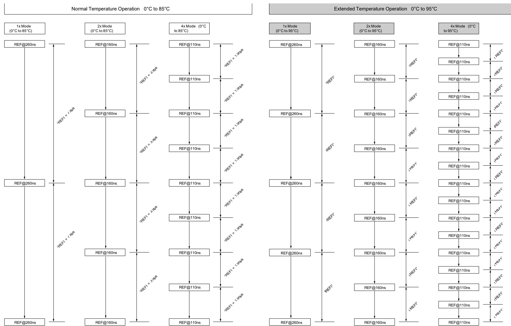
Figure 81: 4Gb With Fine Granularity Refresh Mode Example
