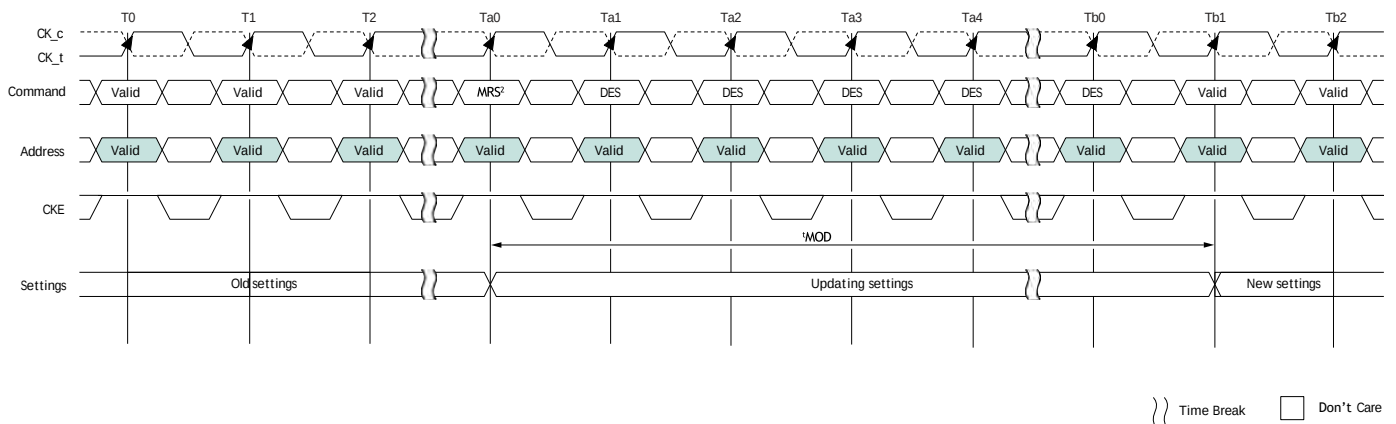
Figure 12: t_{MOD} Timing
