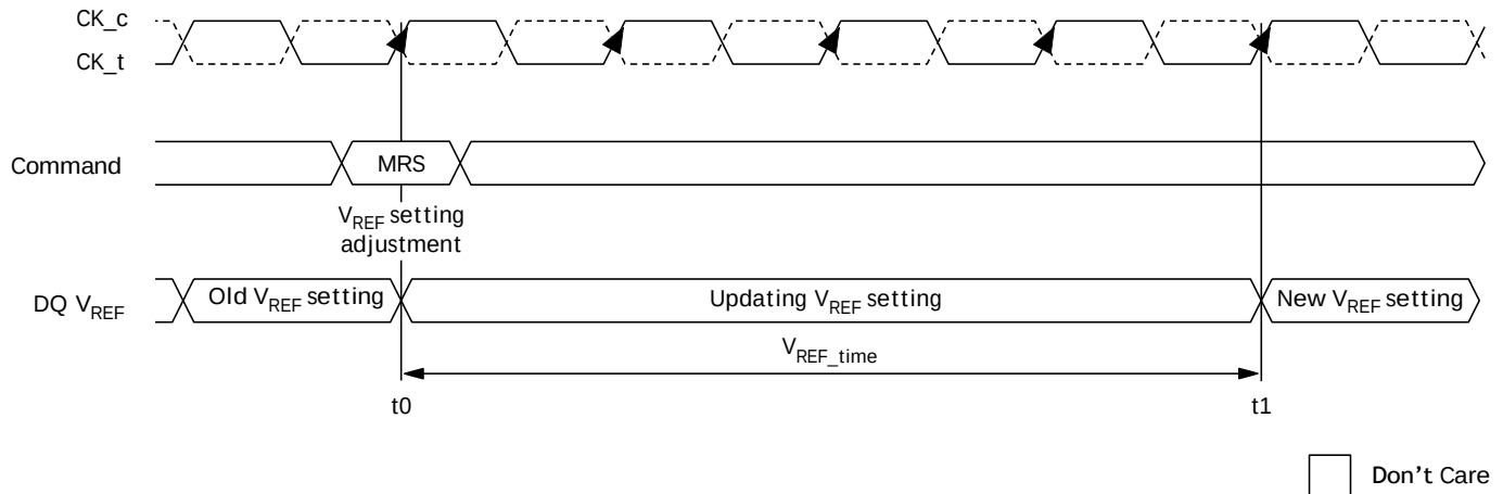
Figure 61: V_{REFDQ} Timing Diagram for V_{REF,time} Parameter
