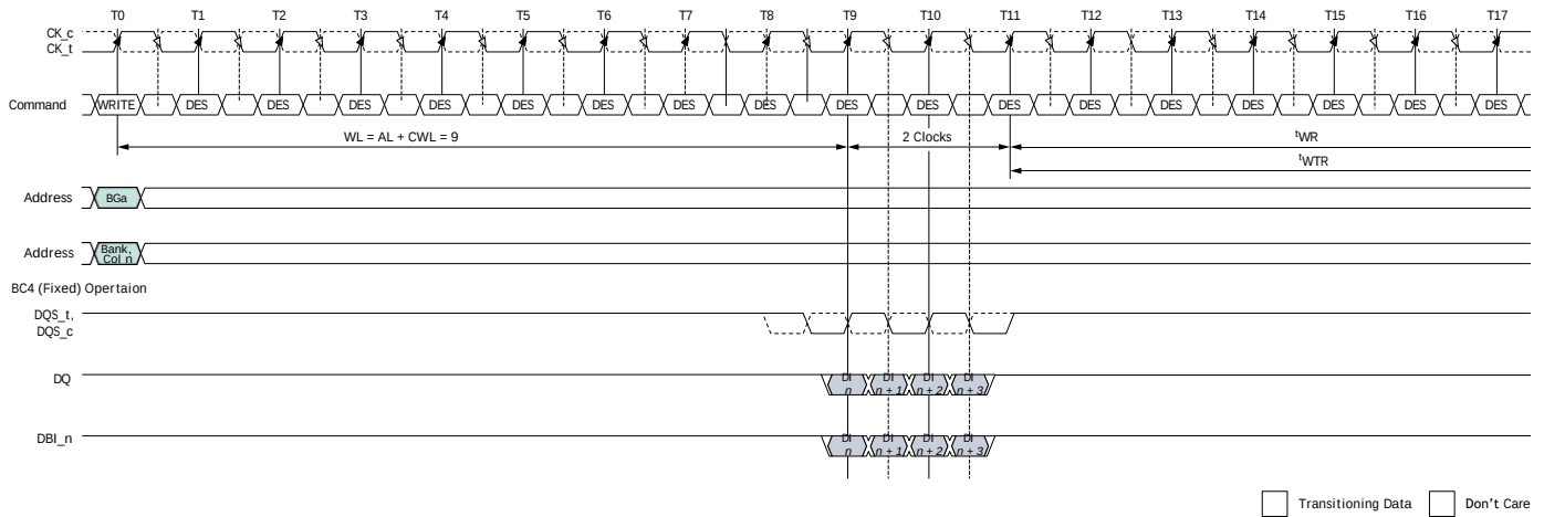
Figure 188: WRITE (BC4-Fixed) with 1^tCK Preamble and DBI
