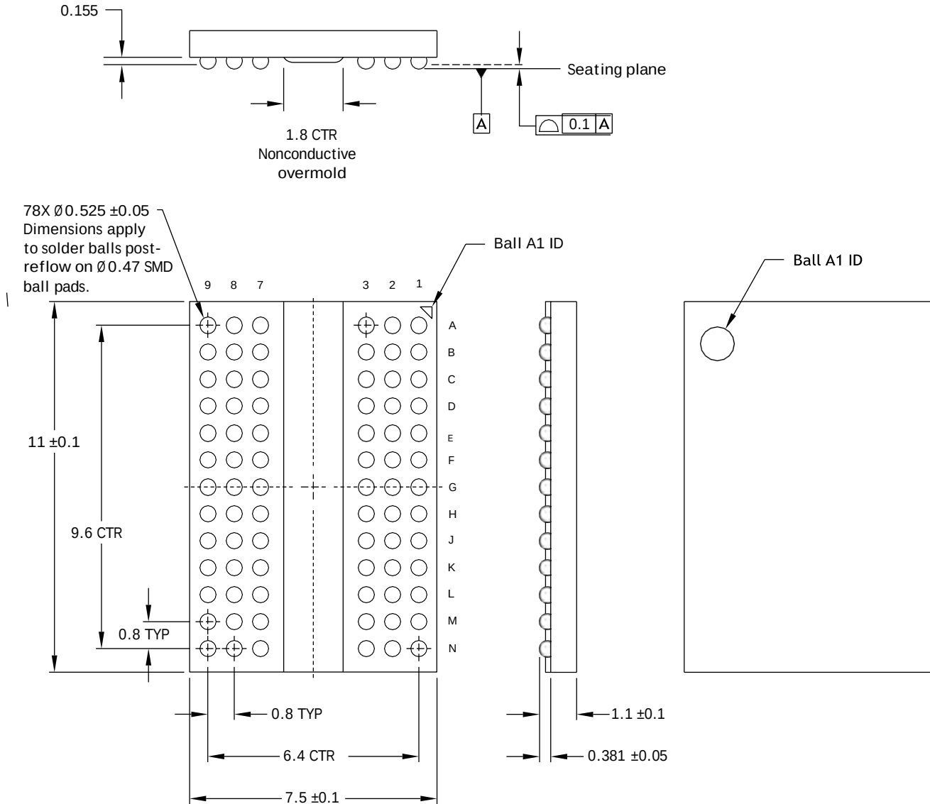
Figure 6: 78-Ball FBGA - x8
