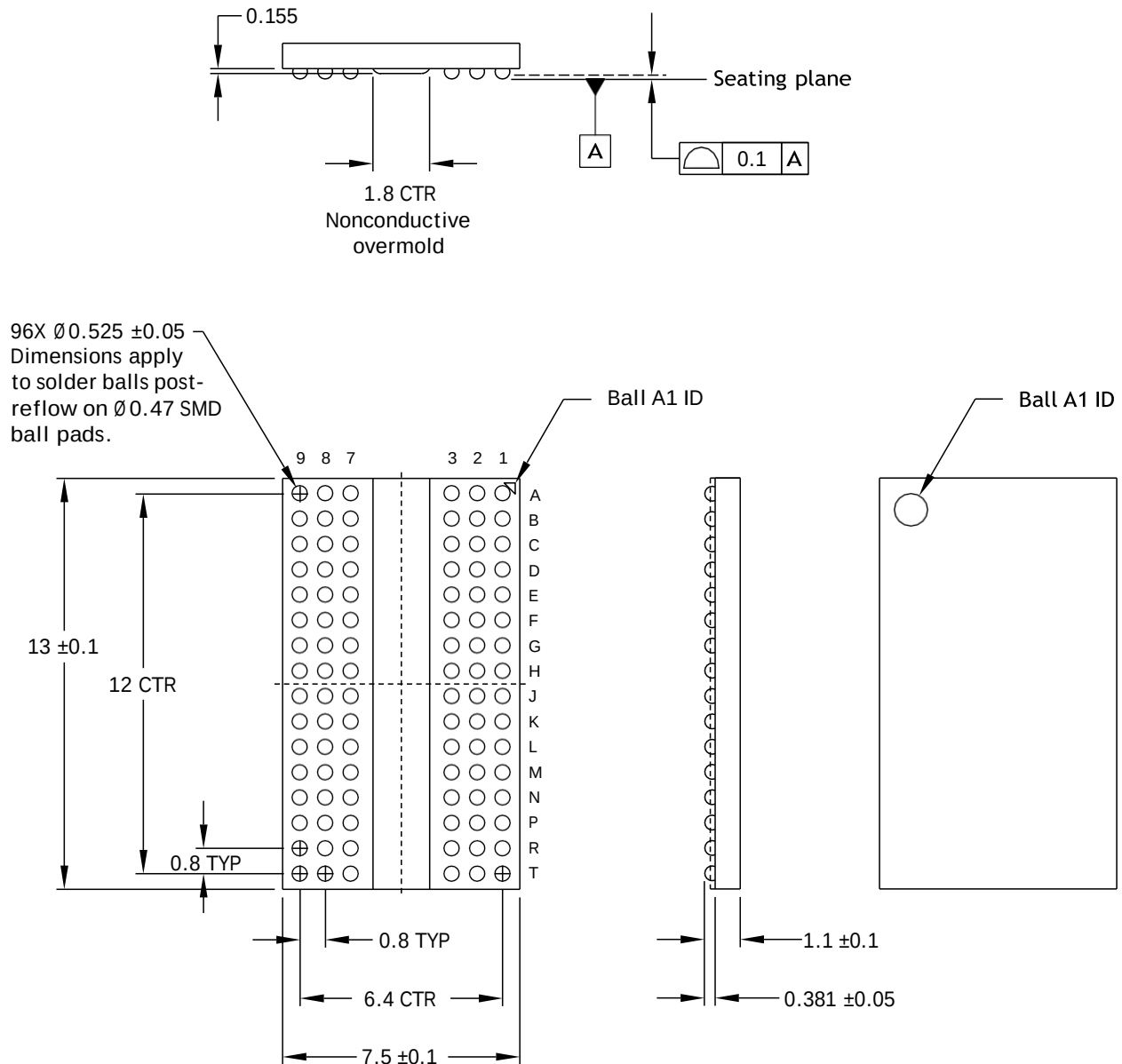
Figure 7: 96-Ball FBGA - x16
