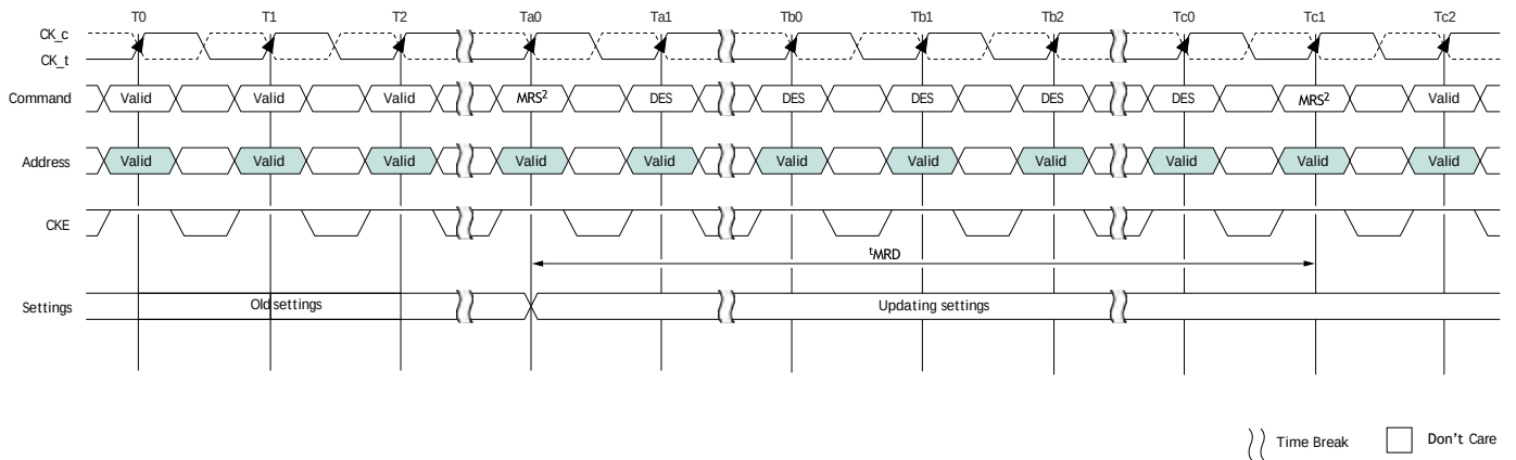
Figure 11: t_{MRD} Timing
