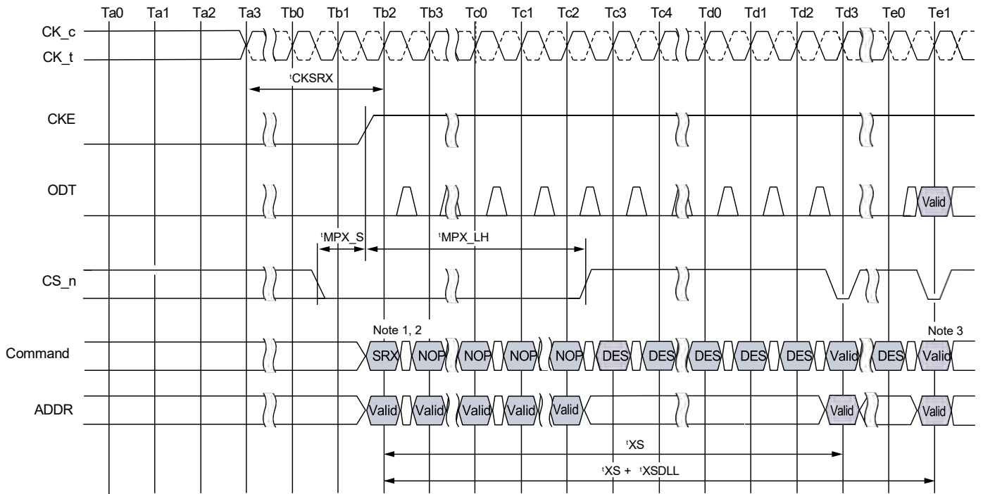
Figure 86: Self Refresh Exit with NOP Command
