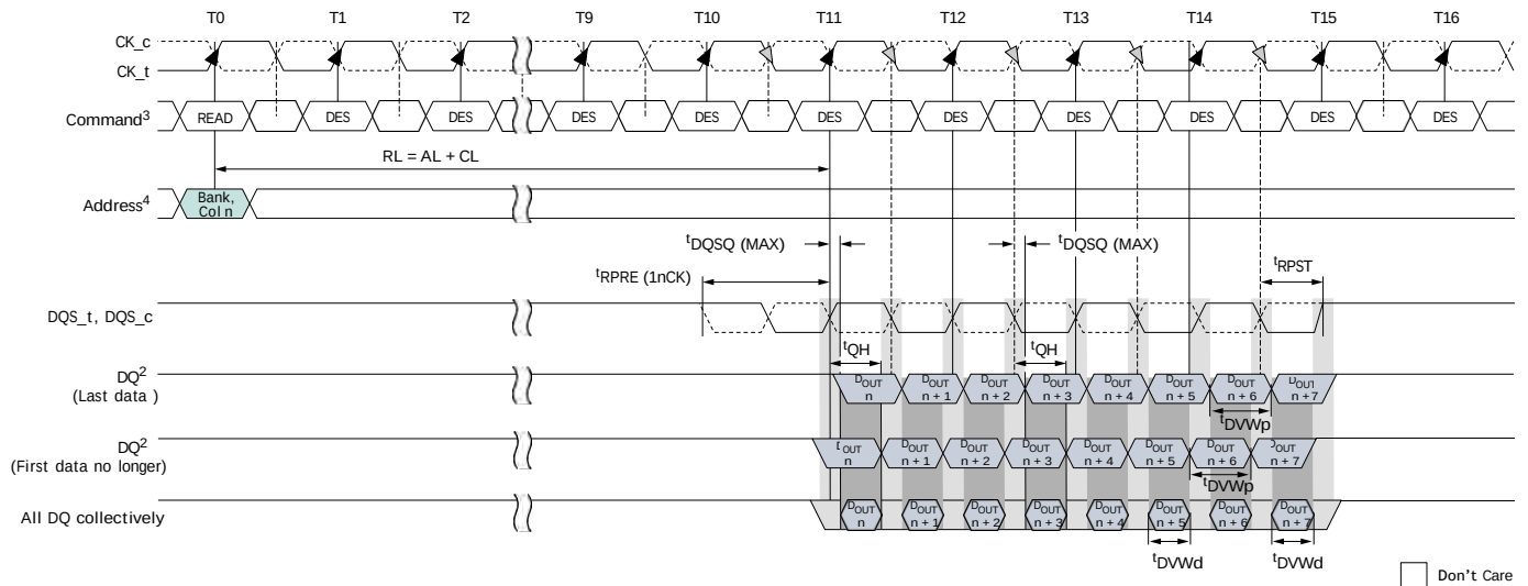
Figure 120: Data Strobe-to-Data Relationship
