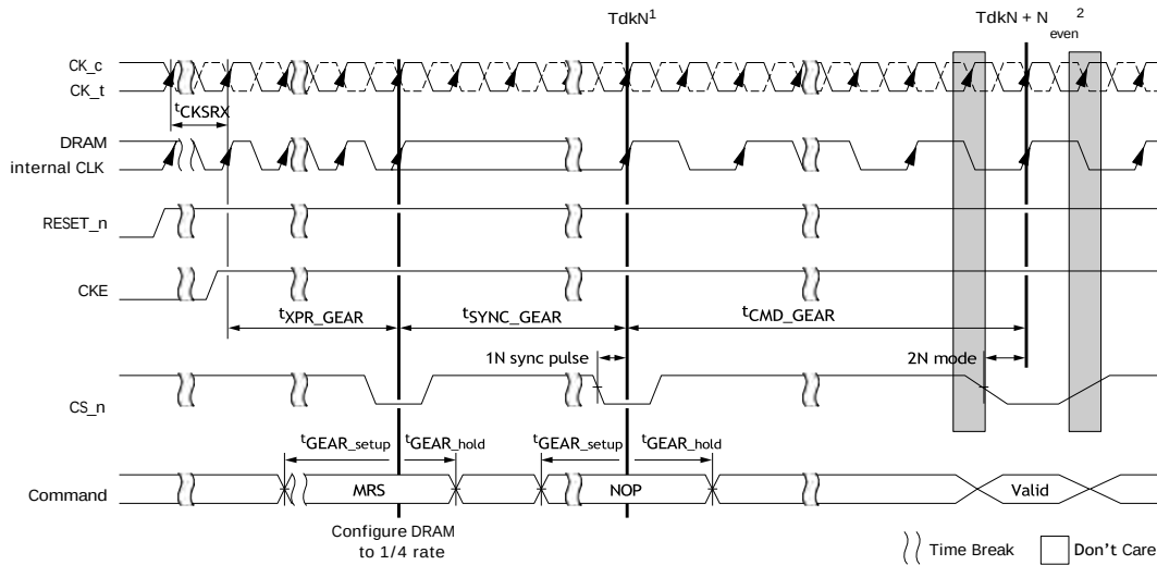
Figure 38: Clock Mode Change from 1/2 Rate to 1/4 Rate (Initialization)
