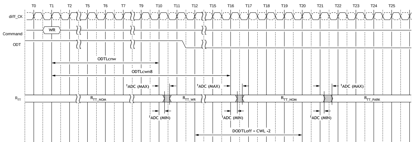
Figure 201: Dynamic ODT Overlapped with R TT(NOM) (CL = 14, CWL = 11, BL = 8, AL = 0, CRC Disabled)
