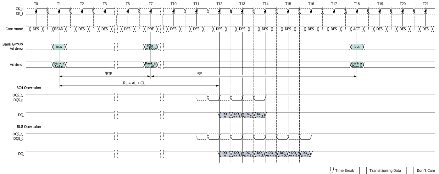
Figure 146: READ to PRECHARGE with 1^t\text{CK} Preamble
