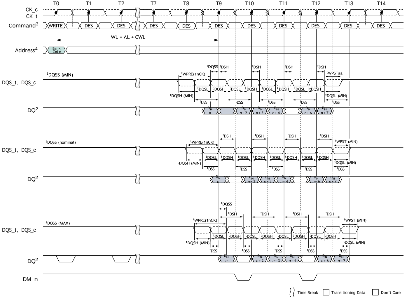
Figure 158: Write Timing Definition
