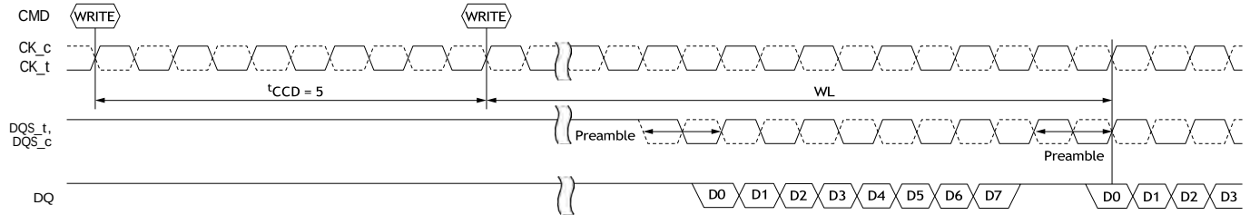
Figure 106: 1 t CK vs. 2 t CK WRITE Preamble Mode, t_{CCD} = 5
