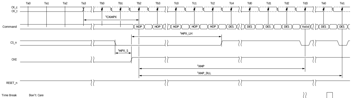
Figure 44: Maximum Power-Saving Mode Exit
