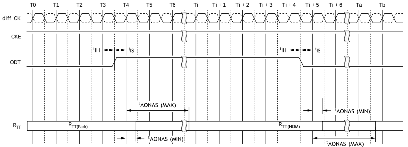
Figure 202: Asynchronous ODT Timings with DLL Off
