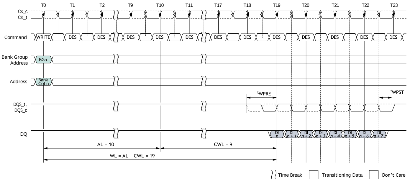
Figure 167: WRITE Burst Operation, WL = 19 (AL = 10, CWL = 9, BL8)
