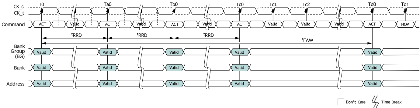
Figure 76: t_{FAW} Timing
