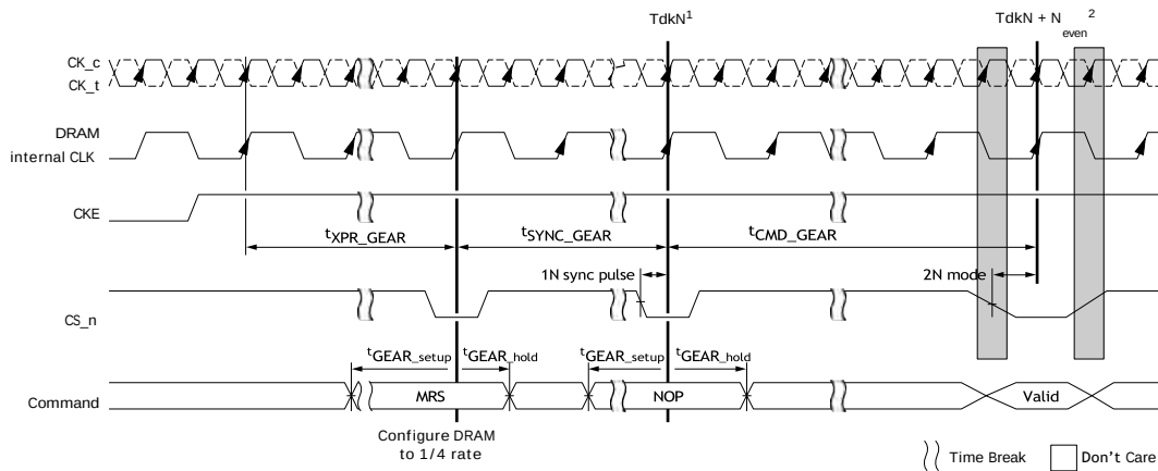
Figure 39: Clock Mode Change After Exiting Self Refresh
