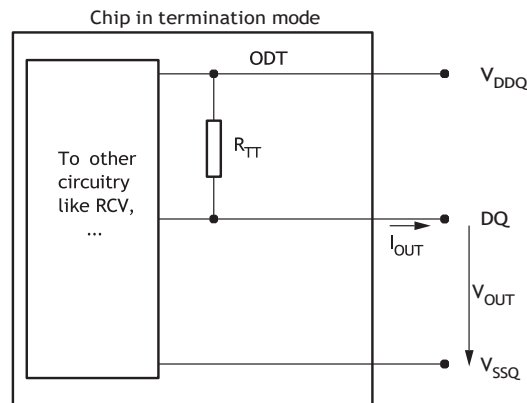
Figure 239: ODT Definition of Voltages and Currents
