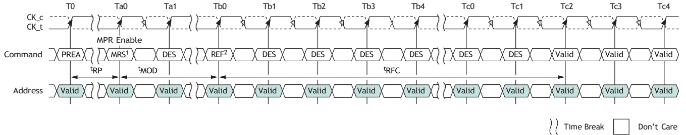
Figure 40: REFRESH Timing
