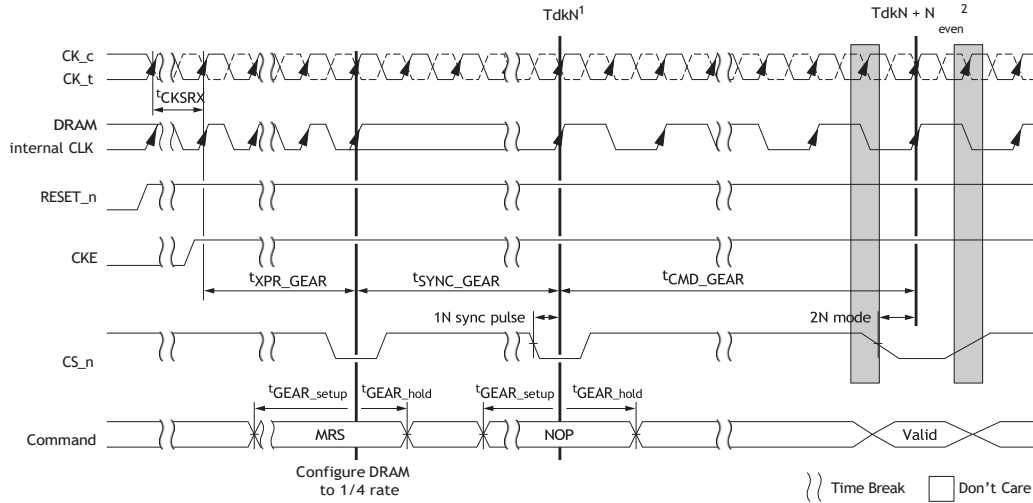
Figure 43: Clock Mode Change from 1/2 Rate to 1/4 Rate (Initialization)
