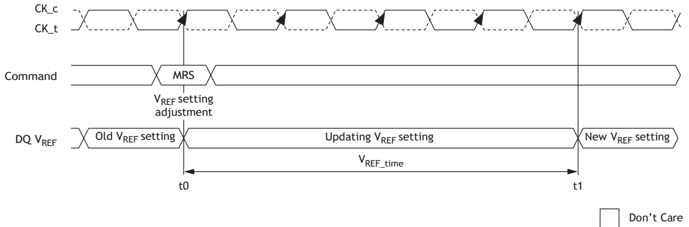
Figure 66: V_{REFDQ} Timing Diagram for V_{REF,time} Parameter
