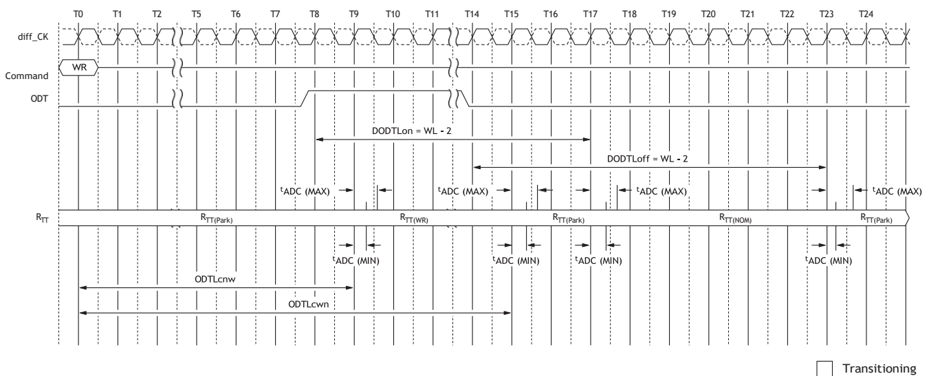
Figure 206: Dynamic ODT (1 st CK Preamble; CL = 14, CWL = 11, BL = 8, AL = 0, CRC Disabled)
