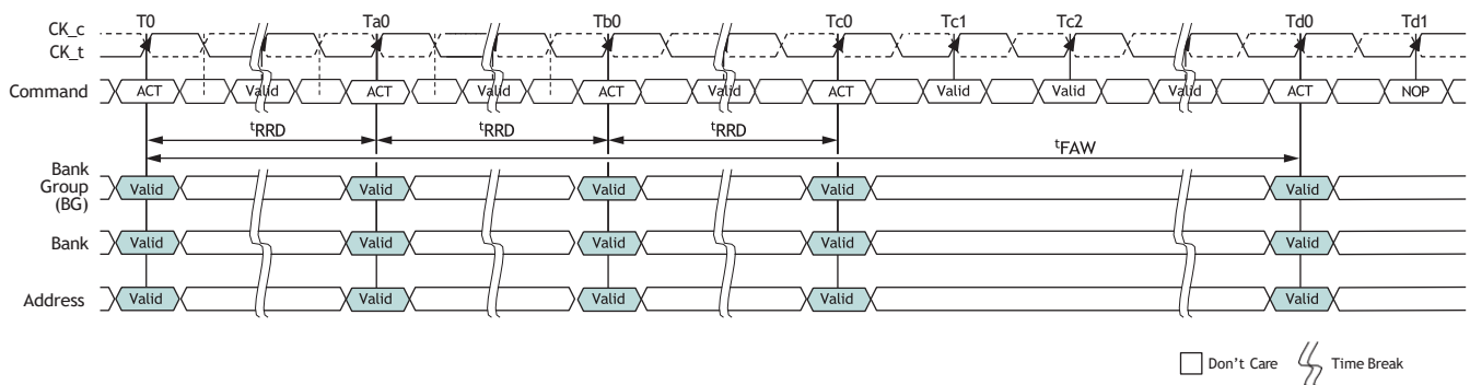
Figure 82: t_{FAW} Timing
