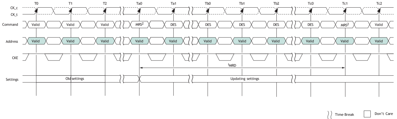
Figure 16: t_{MRD} Timing
