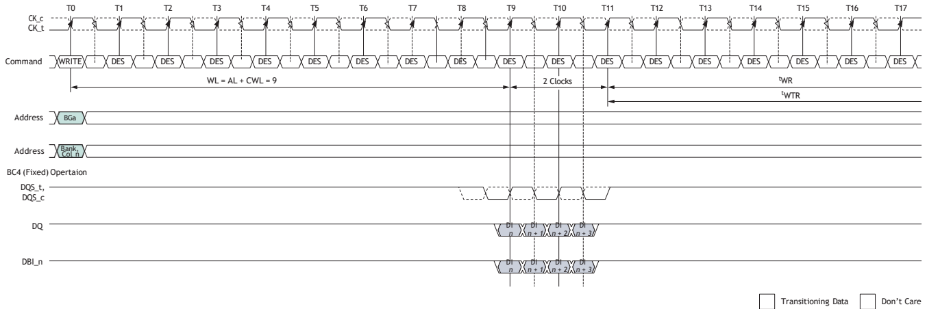
Figure 194: WRITE (BC4-Fixed) with 1t_{CK} Preamble and DBI
