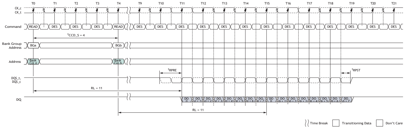
Figure 132: Consecutive READ (BL8) with 1^t\text{CK} Preamble in Different Bank Group
