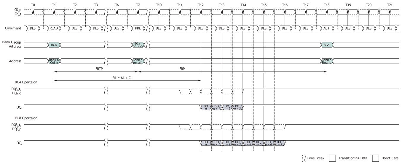
Figure 152: READ to PRECHARGE with 1^{\text{t}}\text{CK} Preamble
