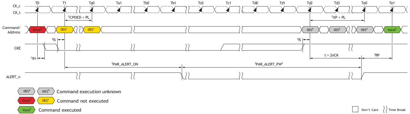
Figure 55: CA Parity Error Checking – PDEIPDX
