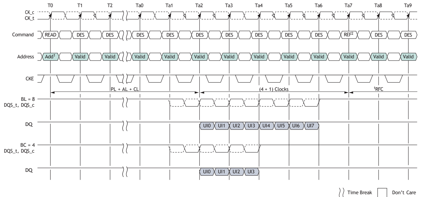
Figure 41: READ-to-REFRESH Timing
