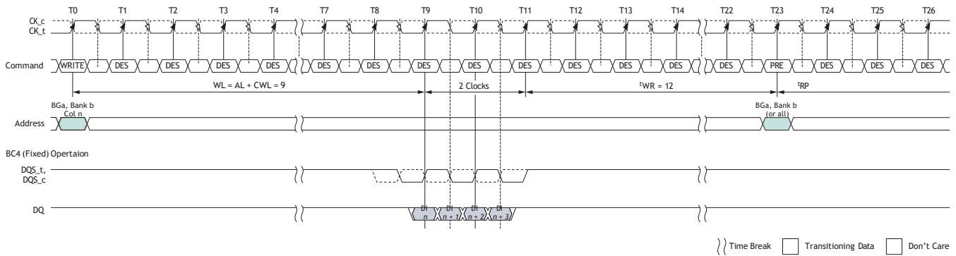
Figure 190: WRITE (BC4-Fixed) to PRECHARGE with 1^t\text{CK} Preamble
