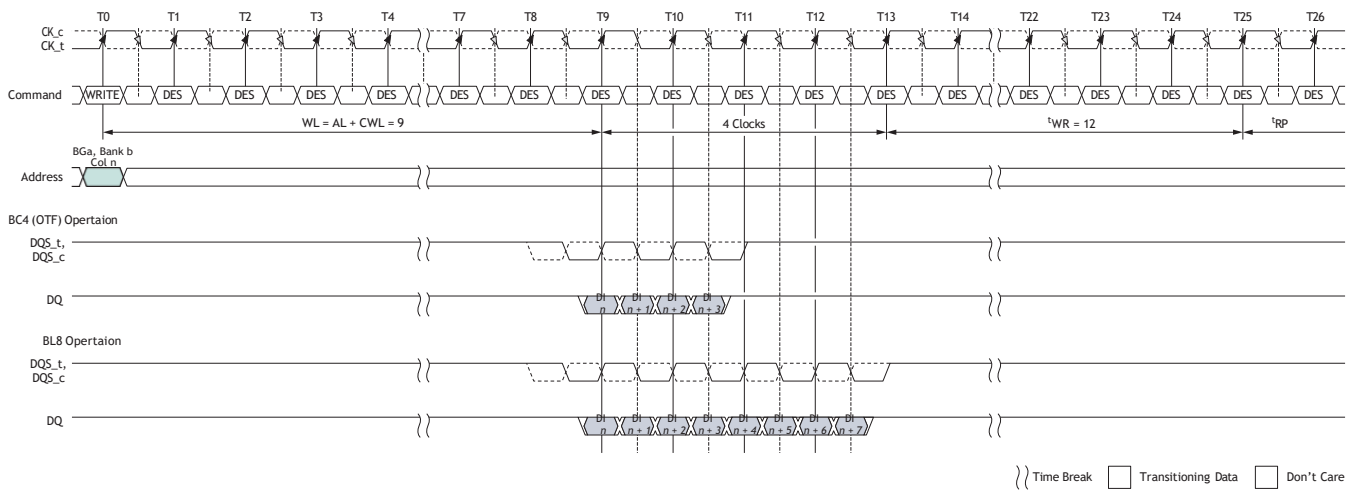
Figure 191: WRITE (BL8/BC4-OTF) to Auto PRECHARGE with 1^t\text{CK} Preamble
