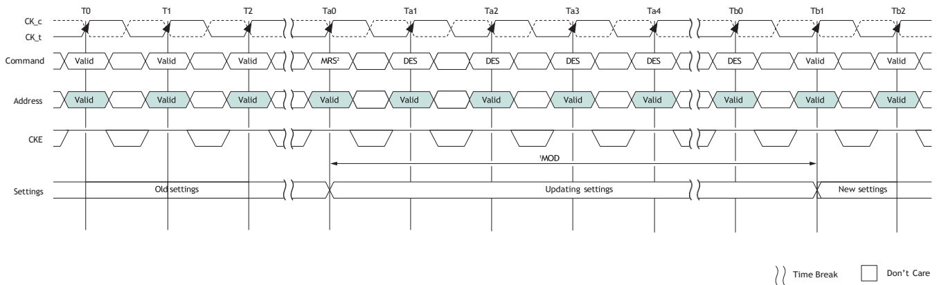
Figure 17: t_{MOD} Timing
