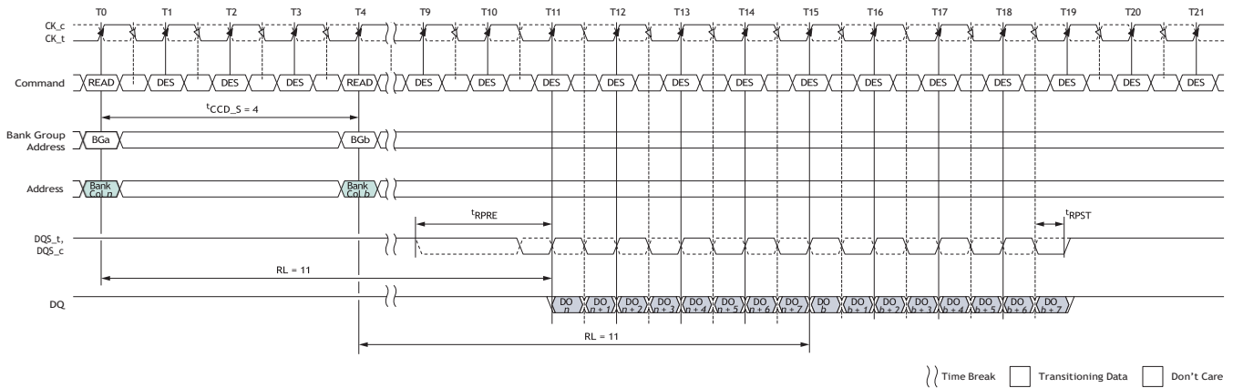
Figure 133: Consecutive READ (BL8) with 2^t\text{CK} Preamble in Different Bank Group
