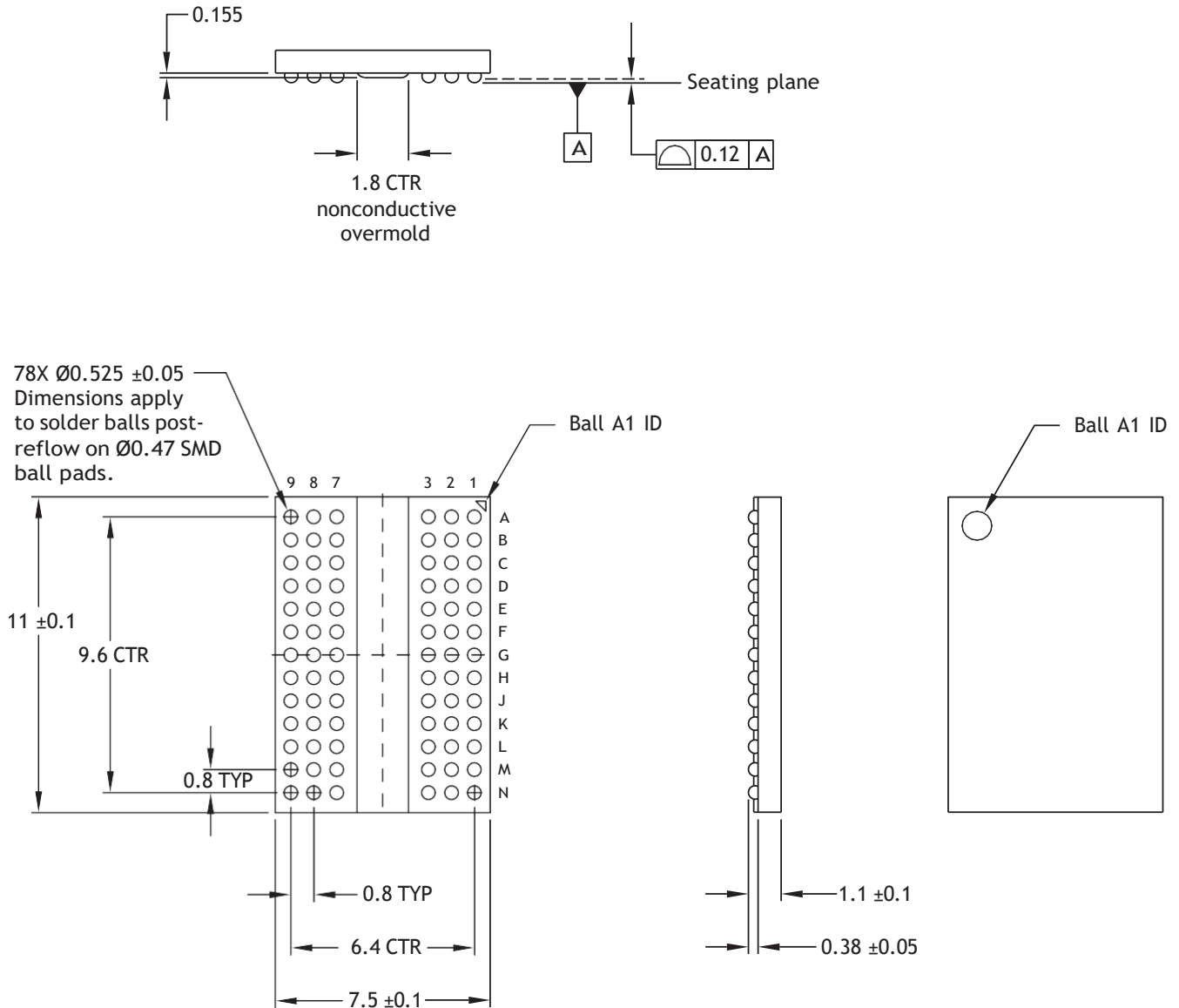
Figure 8: 78-Ball FBGA – x4, x8
