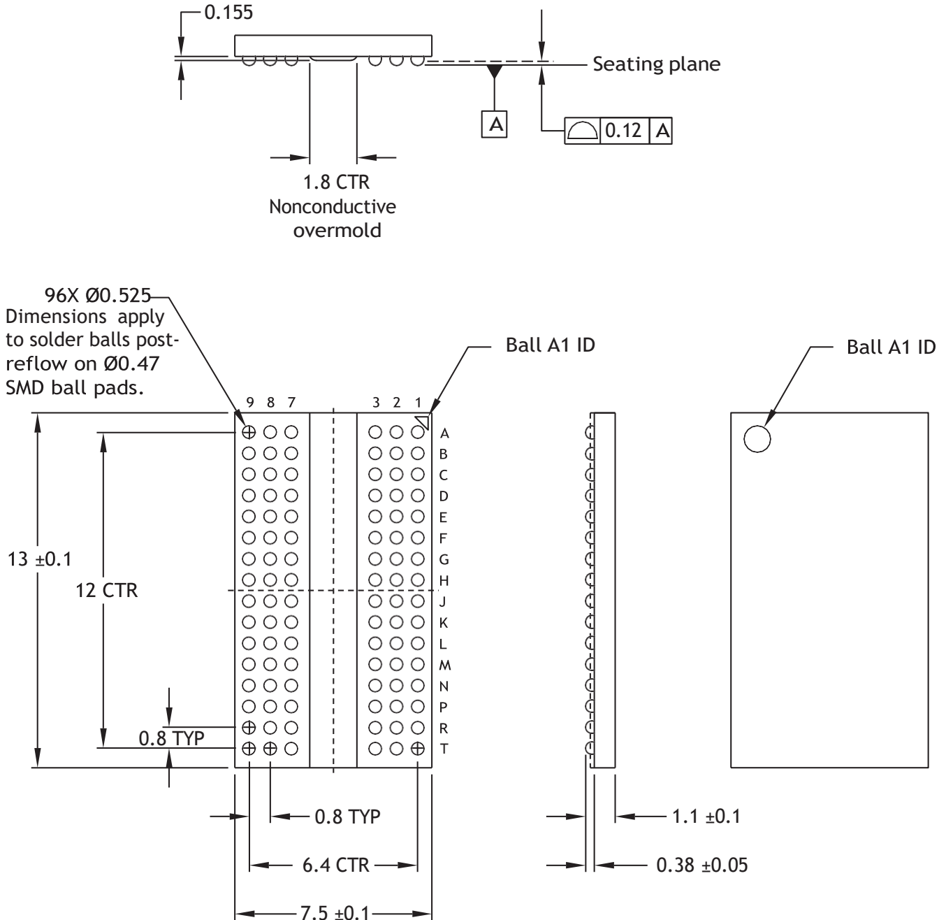
Figure 12: 96-Ball FBGA – x16
