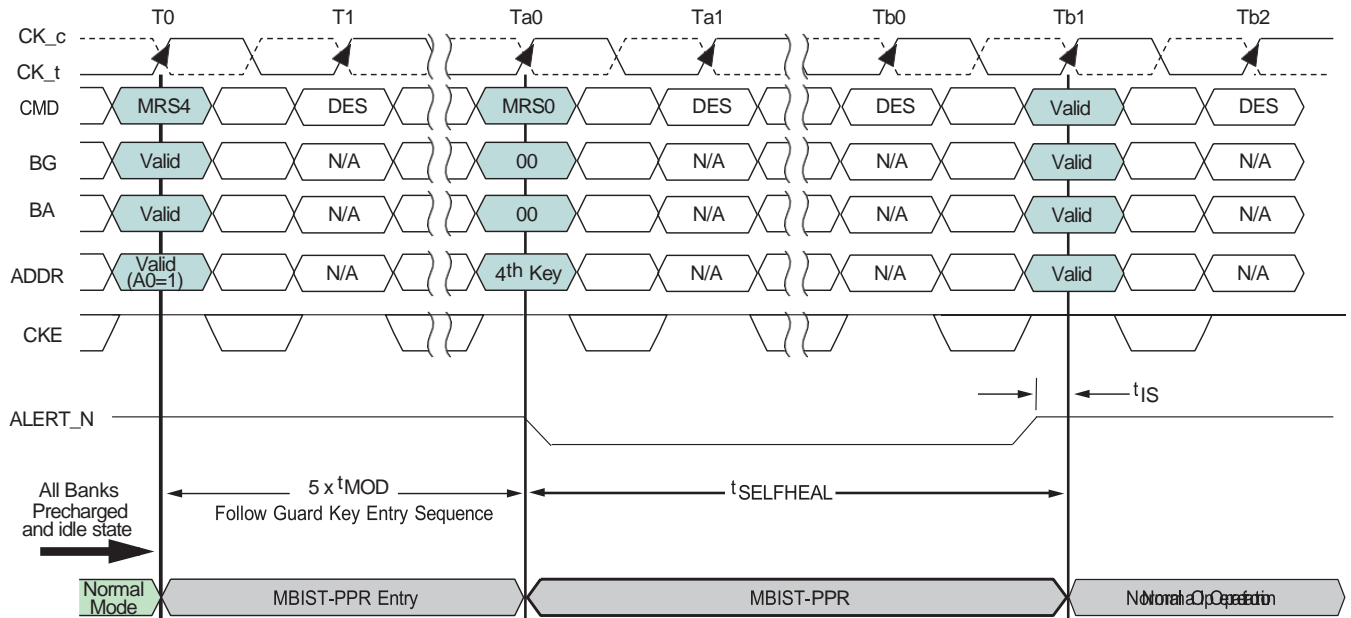
Figure 80: MBIST-PPR Sequence
