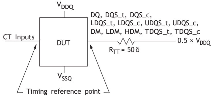
Figure 235: Connectivity Test Mode Output Slew Rate Definition
