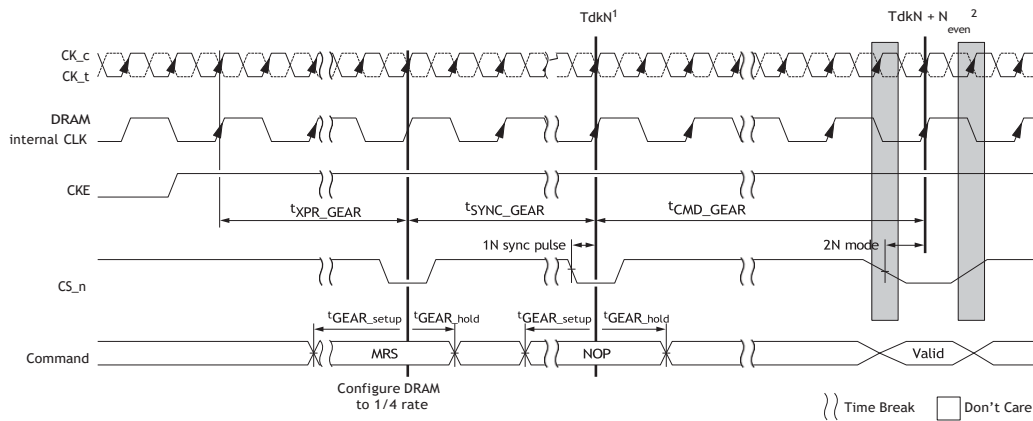
Figure 44: Clock Mode Change After Exiting Self Refresh
