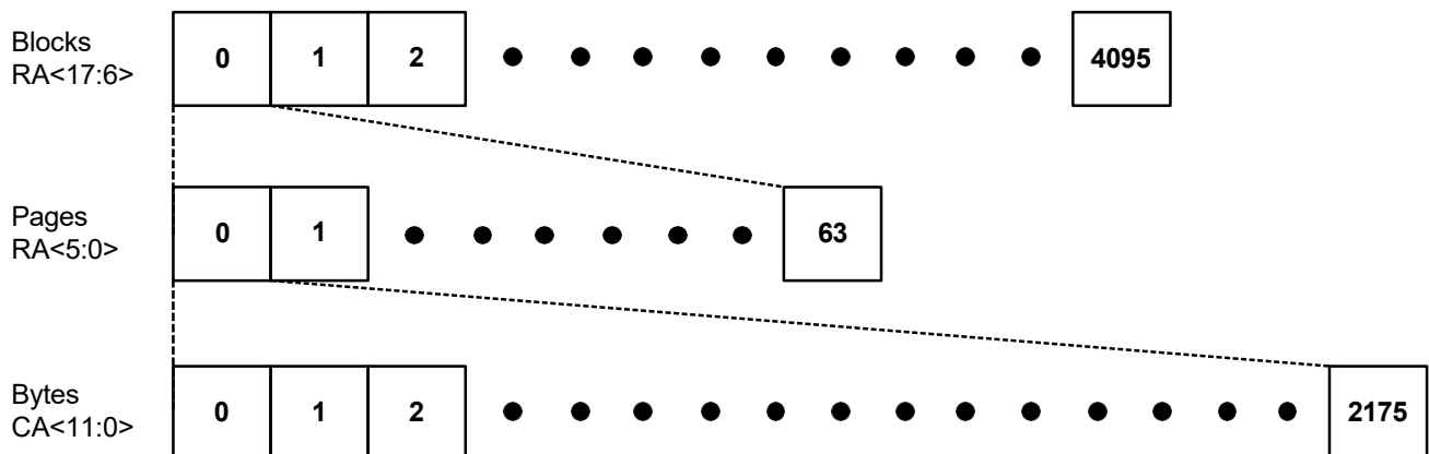
Figure 1-3. Memory Mapping Diagram for AS5F34G04SNDA-08LIN
