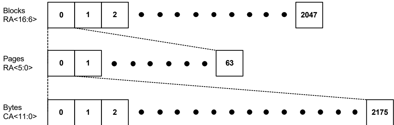
Figure 1-2. Memory Mapping Diagram for AS5F32G04SNDA-08LIN
