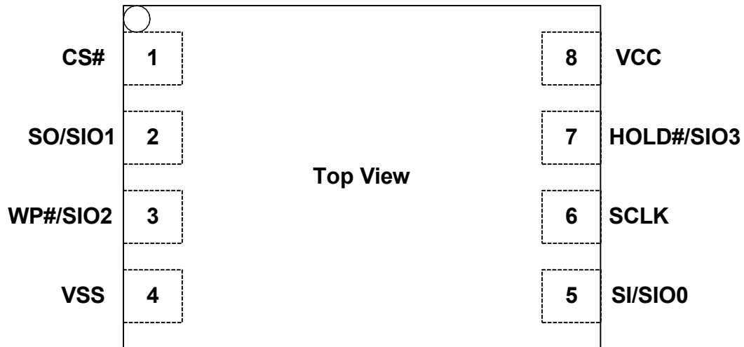
Figure 1-4. Pin Assignments
