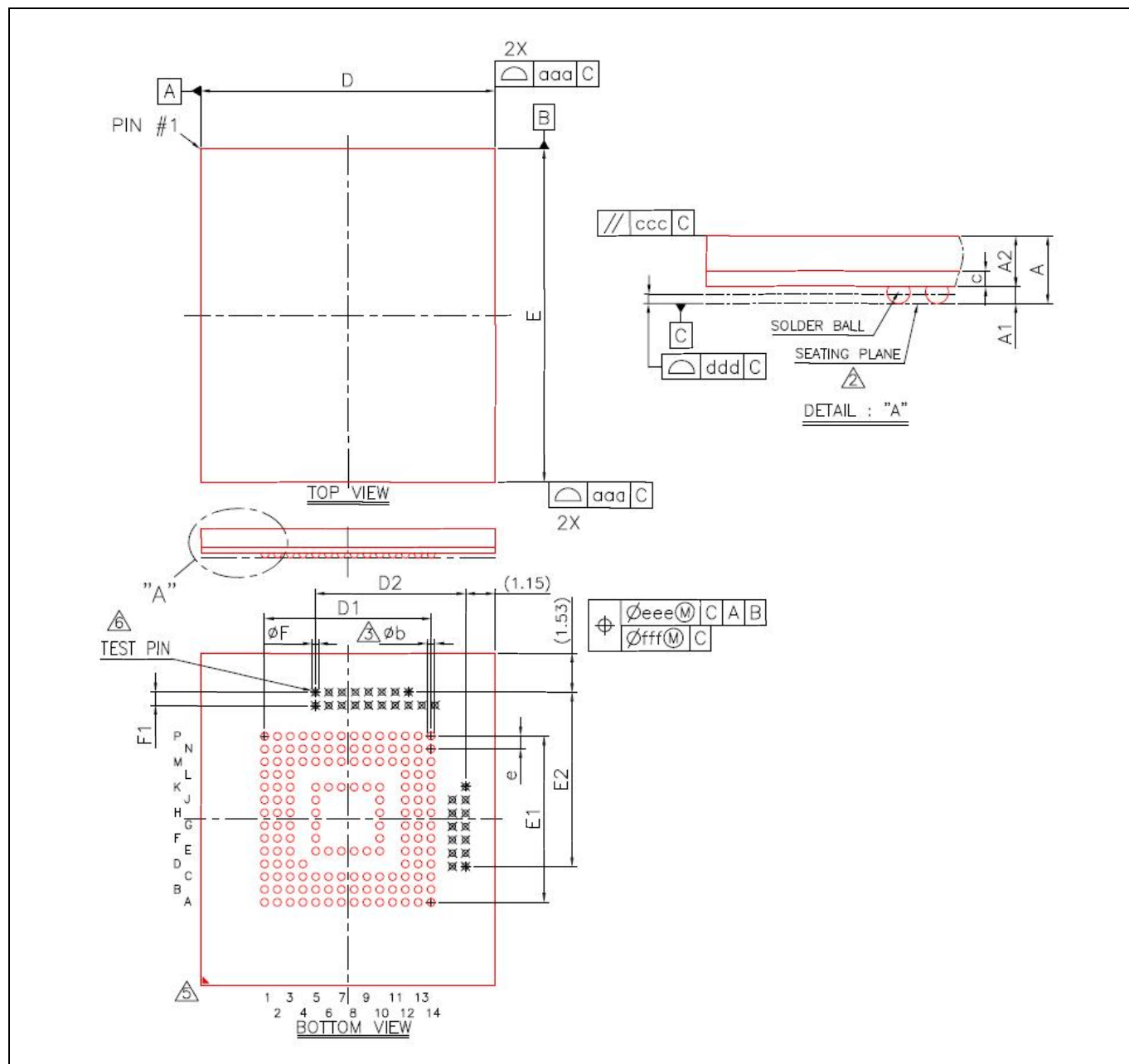
Figure 4: 153-Ball BGA Package Outline (11.5mmx13mmx1.2mm)
