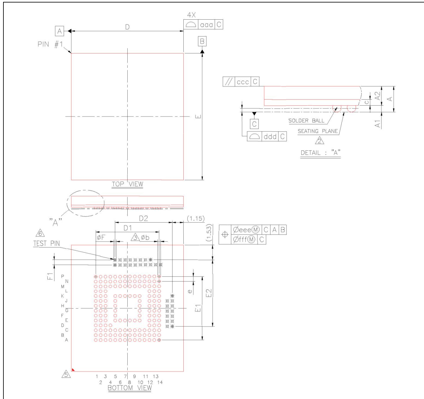
Figure 5: 153-Ball BGA Package Outline (11.5mmx13mmx1.4mm)
