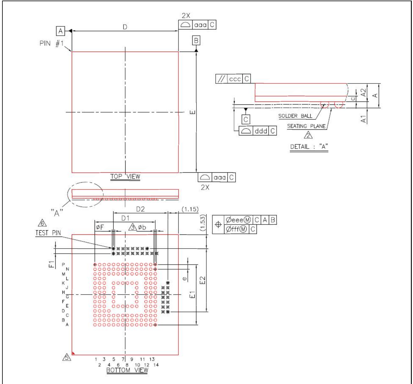
Figure 4: 153-Ball BGA Package Outline (11.5mmx13mmx1.2mm)
