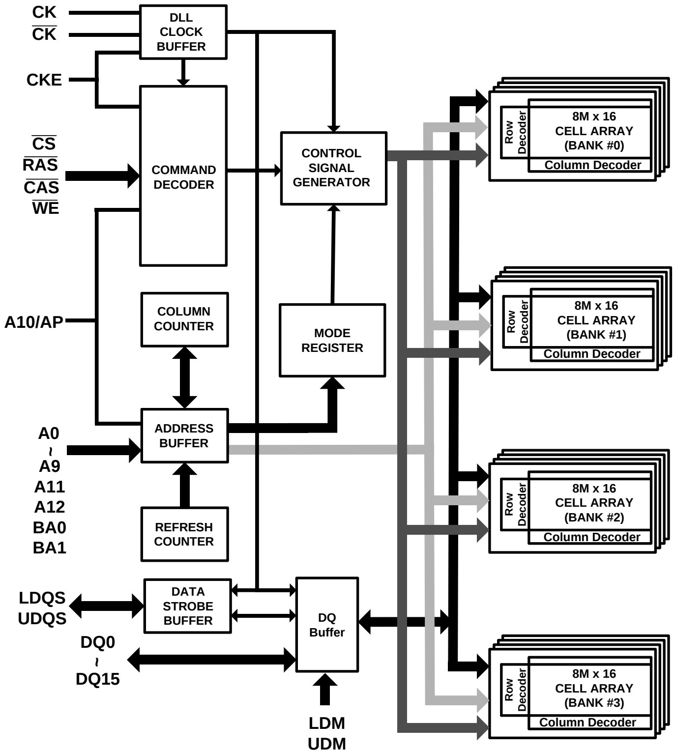
Figure 2. Block Diagram
