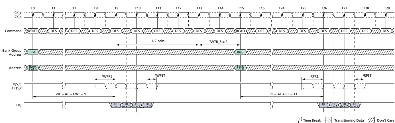
Figure 179: WRITE (BC4) OTF to READ (BC4) OTF with 1^{\text{t}}\text{CK} Preamble in Different Bank Group
