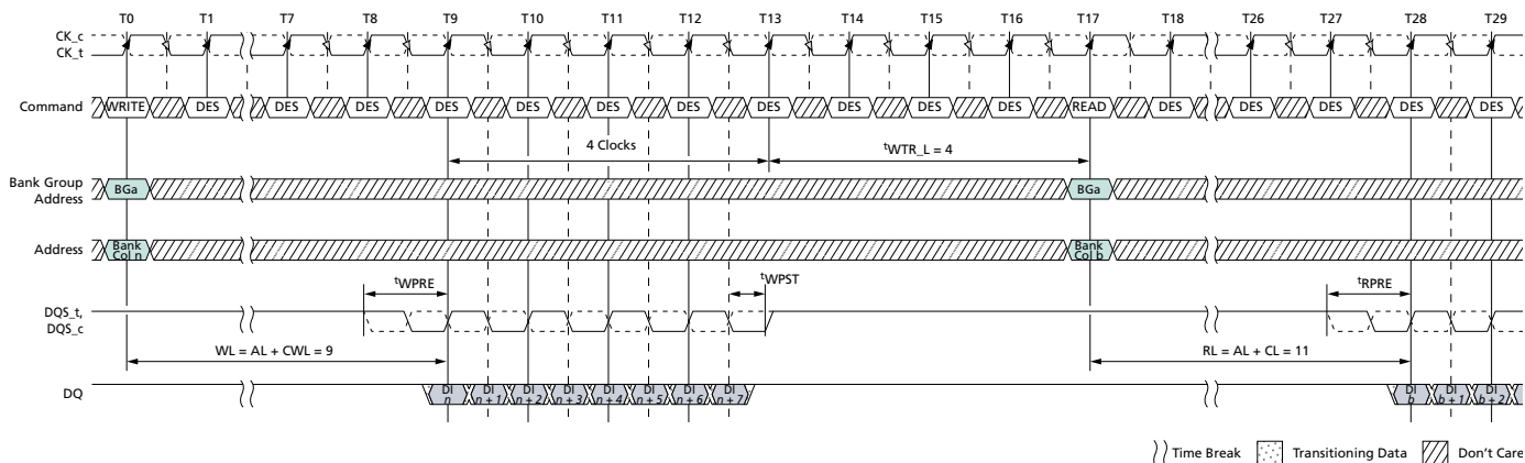
Figure 178: WRITE (BL8) to READ (BL8) with 1^{\text{t}}\text{CK} Preamble in Same Bank Group
