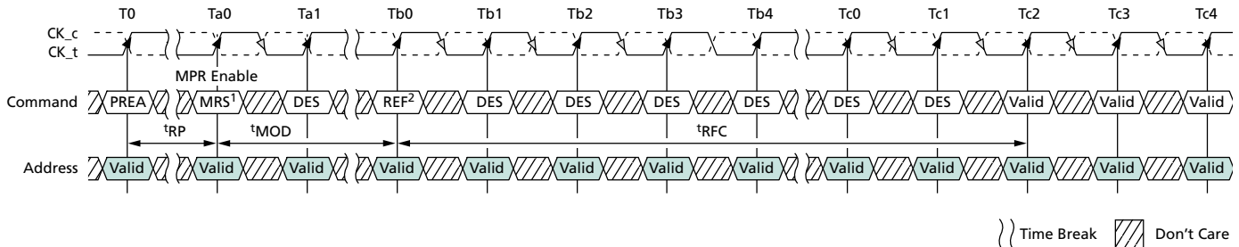
Figure 35: REFRESH Timing
