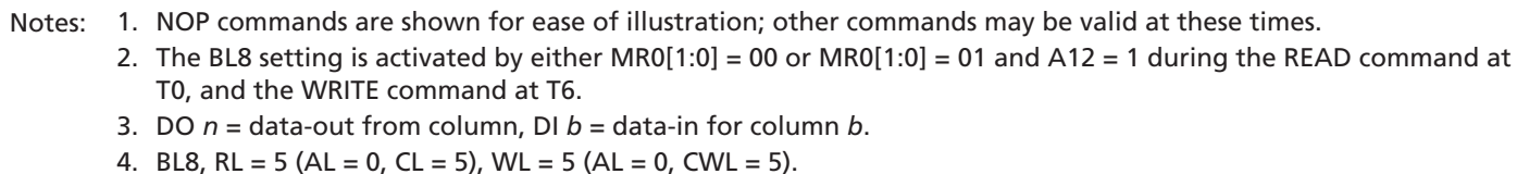
2Gb: x4, x8, x16 DDR3 SDRAM READ Operation
