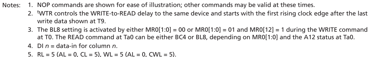
2Gb: x4, x8, x16 DDR3 SDRAM WRITE Operation
