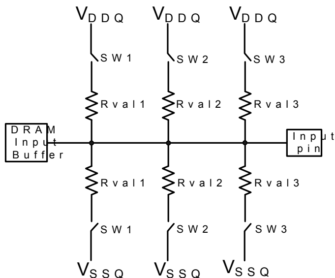
Figure 4. Functional representation of ODT
