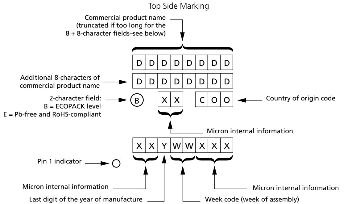
Figure 16: DFN/6x5 V2 Component Marks, Package Option:F6, F7 and W7
